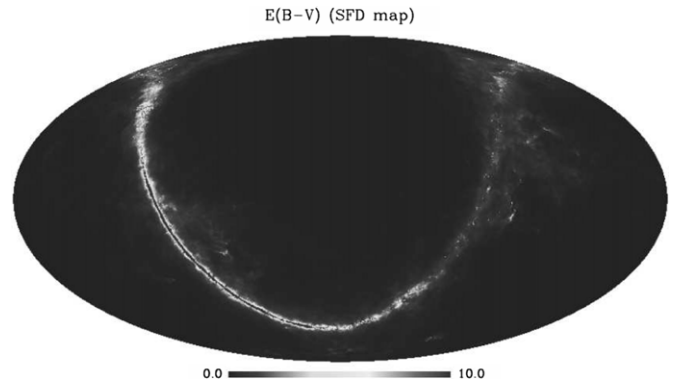
Figure 17. Galactic extinction map from Schlegel et al. (1998). By comparing with the full mask of the sky, we can see that for regions of maximum extinction, the Galactic plane is completely avoided.
