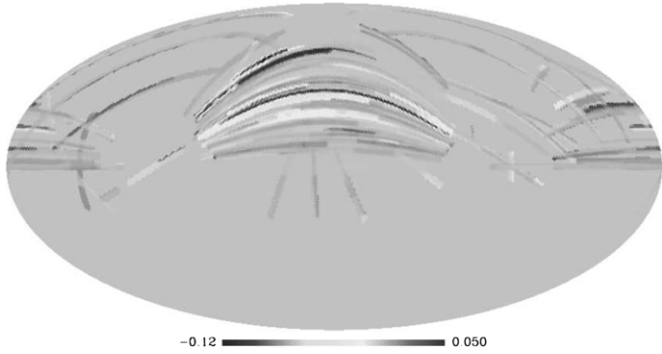
Figure 19. Color offsets in r-i calculated from sources provided by Schlafly et al. (2010). These are derived from the spectra of the stars, and thus do not include an intrinsic variation due to the metallicity gradient of stars within our Galaxy.
