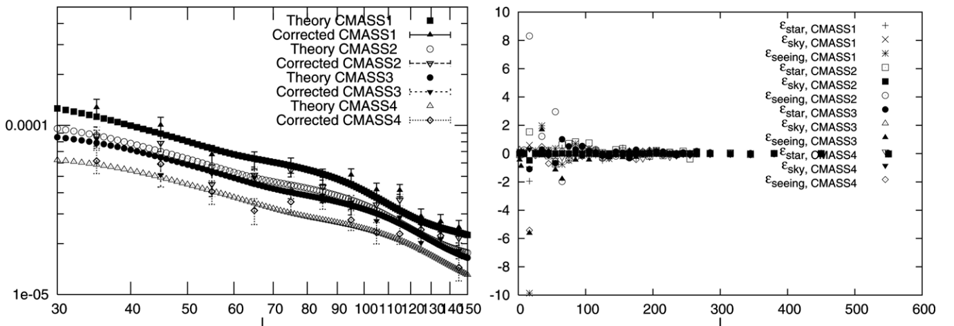
Figure 24. For the first plot, we show the systematic-corrected power spectra and their corresponding best-fit model (from flat \Lambda CDM model) when we include all three dominant systematics (stars, sky, and seeing). For the last plot, we included the measured \epsilon (as described in Equation (18)) for all the dominant systematics.
