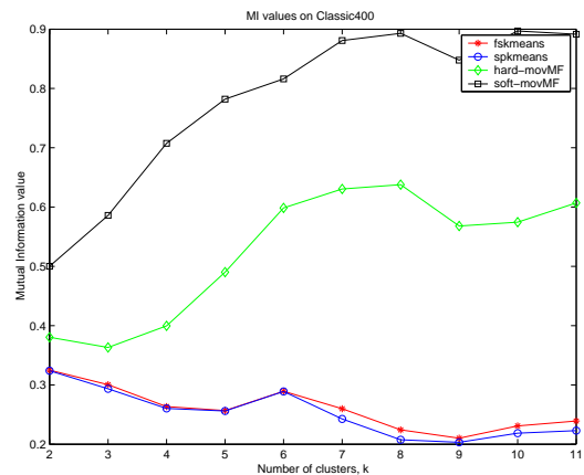
(c) Comparison of MI values for Classic400.
