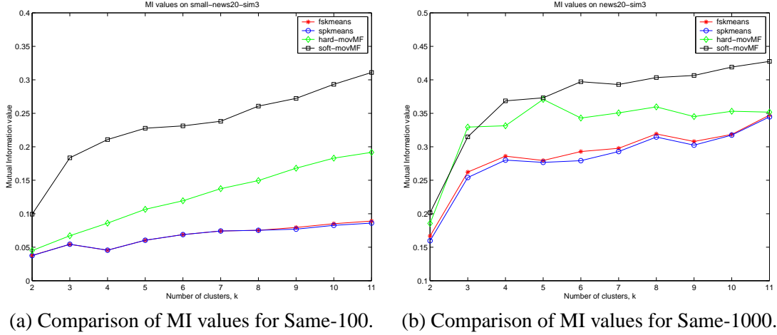
Figure 4: Comparison of the algorithms for more subsets of CMU Newsgroup data.
