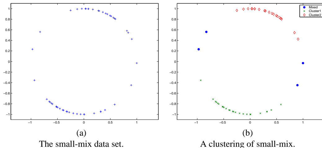
Figure 1: Small-mix data set and its clustering by soft-moVMF .
