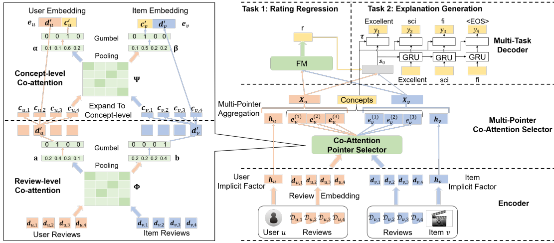
Figure 2: Framework of the proposed model for explainable recommendation.
