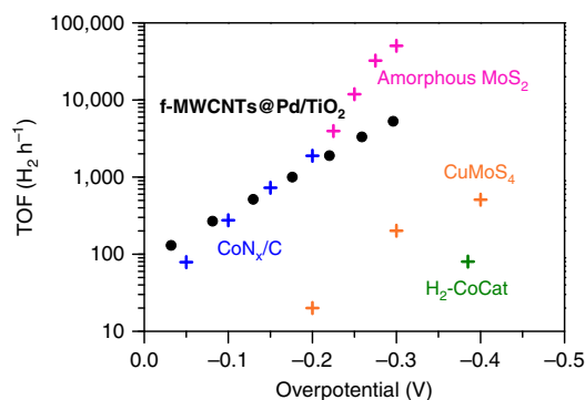
Figure 4 | Comparison of mass-normalized TOF with other catalysts.
