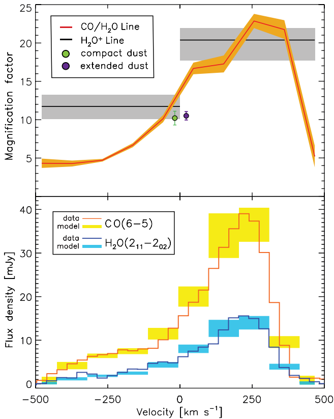
Fig. 7. Top panel: magnification factor as a function of velocity for the emission lines of CO, H 2 O, and H 2 O + , and indicated for the two dust components (the legend at the top left corner indicates the line and point style for each component of emission). Bottom panel: a comparison between the integrated spectrum of the observations and lens-model reconstructed data seen in the image plane. The filled regions show the model reconstructed using the bins in the image-plane spectra, while the histogram lines show the observed image-plane spectra (see the legend at the top left). The model overall predicts very well the spectra in the source plane.
