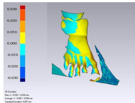
Figure 1. 3D comparison of TLS and LS registered data.
