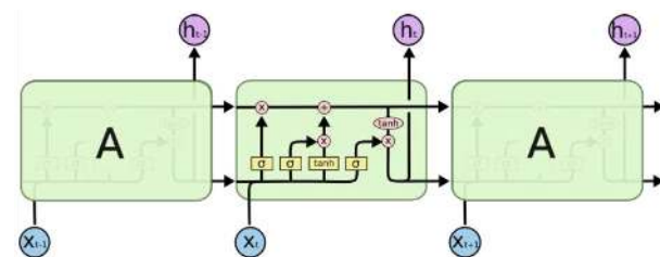
FIGURE 4. LSTM architecture.
