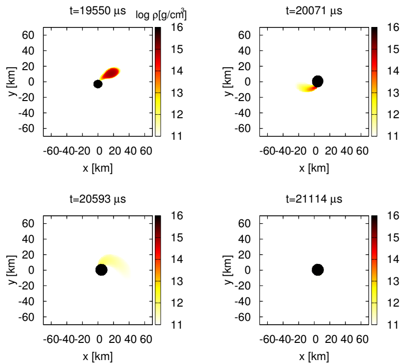
Figure 12: The same as Figure 11 but for a model with M_{\text{BH}} = 4.05 M_{\odot} , a = 0 , M_{\text{NS}} = 1.35 M_{\odot} , and R_{\text{NS}} = 11.0 \text{ km} (EOS B).
