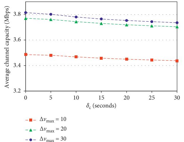
FIGURE 12: Average channel capacity based on the variation of \delta_c and \Delta v_{\max} .
