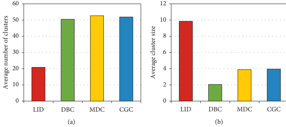
FIGURE 13: Cluster structure based on the number of clusters and cluster size. (a) Average number of clusters and (b) average size of cluster.
