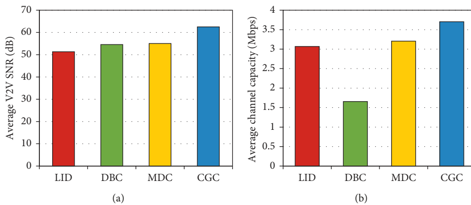
FIGURE 15: Link quality based on V2V SNR and channel capacity. (a) Average V2V SNR and (b) average channel capacity.
