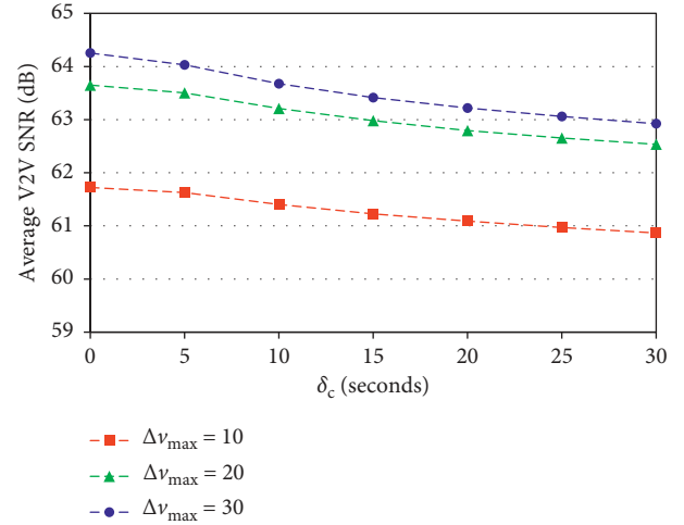
FIGURE 11: Average V2V SNR based on the variation of \delta_c and \Delta v_{\max} .
