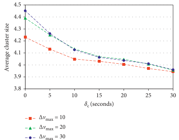
FIGURE 8: Average cluster size based on the variation of \delta_c and \Delta v_{\max} .
