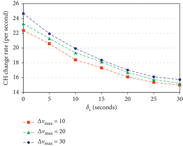
FIGURE 9: Cluster head change rate based on the variation of \delta_c and \Delta v_{\max} .
