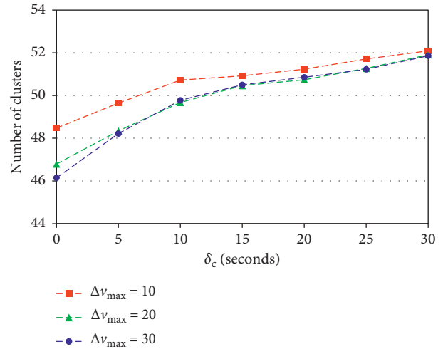
FIGURE 7: Number of clusters based on the variation of \delta_c and \Delta v_{\max} .
