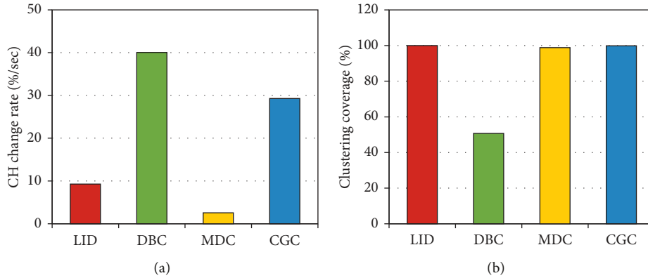
FIGURE 14: Cluster head change rate (a) and clustering coverage (b).
