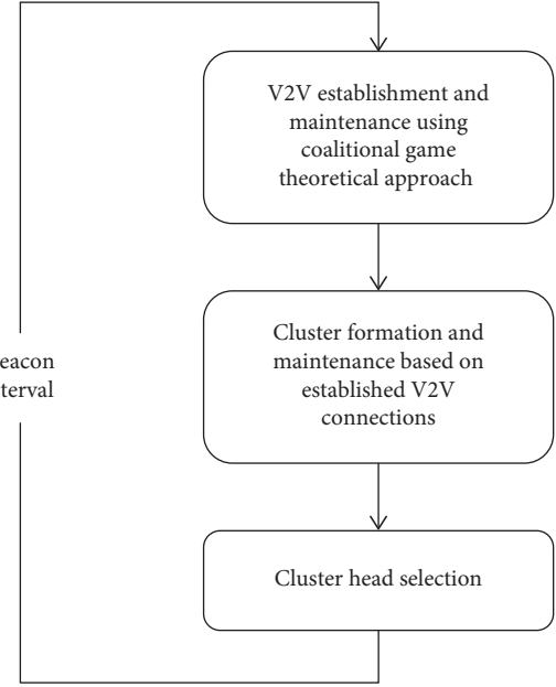
FIGURE 1: Procedure in the proposed clustering method.
