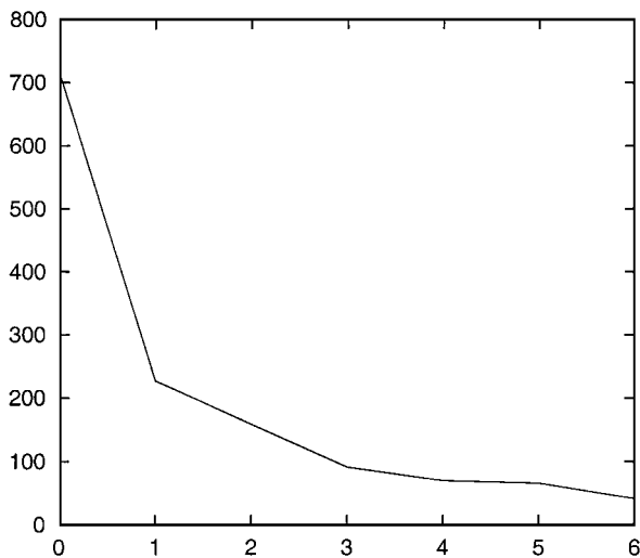
Figure 17. The number of alarms (detections) as a function of the depth m of focusing in pose space. The value corresponding to m is the number of blocks surviving past the m 'th partition.
