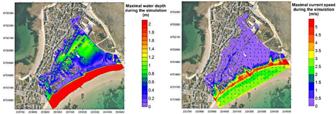
Figure 11. Maximum water depths (left) and currents (right) obtained inland during the SURF-WB simulation on the DEM (with explicit representation of the buildings).
