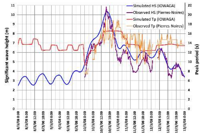
Figure 5. Validation of the wave characteristics simulated in the IOWAGA project on the Pierres-Noires gauge (observation from http://candhis.cetmef.developpement-durable.gouv.fr ).
