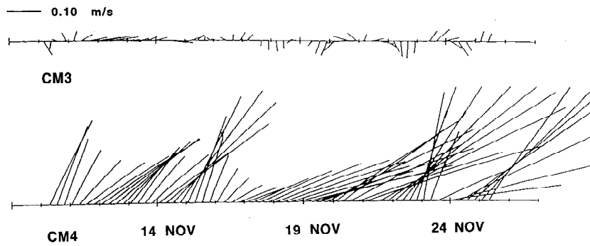
Figure 2a. Temporal variations in the current vectors at 25 m depth at CM3 and CM4 (locations marked in Figure 1b).
