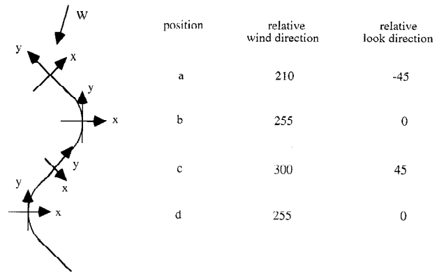
Figure 10. Simplified two-dimensional representation of a meandering front with crest in position d and the trough in position b. The wind direction is marked W . The local coordinate system, along with corresponding relative wind direction and relative look direction measured counterclockwise from the x axis, is listed for four positions along the front. The magnitudes of current shear and convergence/divergence are listed in Table 1.
