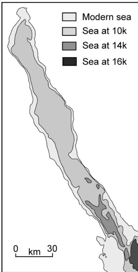
Figure 6. Shoreline positions in the Gulf of Suez at different dates in the most recent sea-level cycle (data compiled by K. Lambeck; drawn by G. Bailey).
