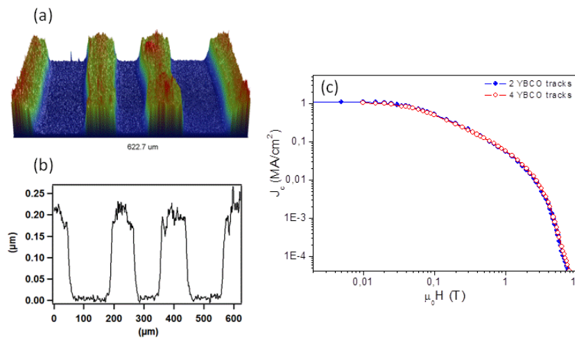
Figure 20. (a) and (b) Optical micrographs and interference profilometry profiles of YBCO patterns prepared by IJD having an average thickness of 200 nm and a width of 200 \mu\text{m} [41]; (c) magnetic field dependence of the critical current density ( J_c ) measured for two tracks (closed symbol) and four tracks (opened symbol) of YBCO films prepared by IJD; reprinted from [42], © 2013, with permission from Elsevier.
