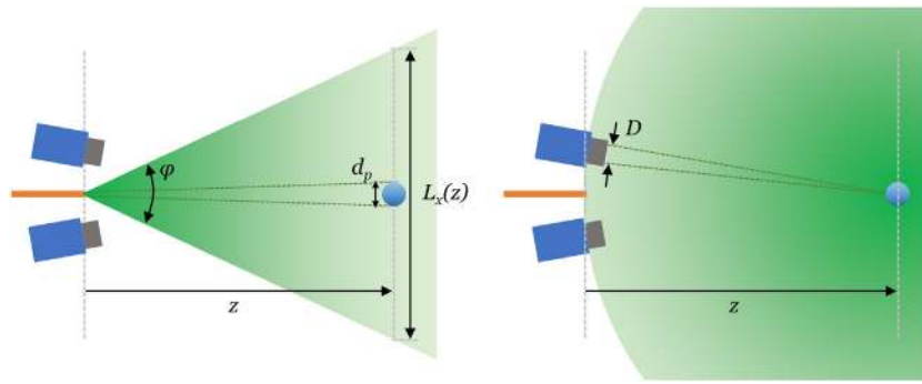
Figure 3. Schematic illustration of laser light propagated from the optical fiber, interacting with a tracer particle (left) and collected back by the cameras (right). Arrangement of optical fiber (orange) in between the cameras (blue) for illustration purposes. Tracer particle not drawn to scale.
