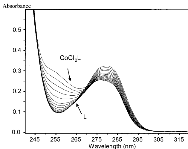
Figure 4. Variation of the absorption spectra observed during the spectrophotometric titration of [L] = 9.51 × 10 −5 M with [CoCl 2 ·6H 2 O] = 1.01 × 10 −3 M
