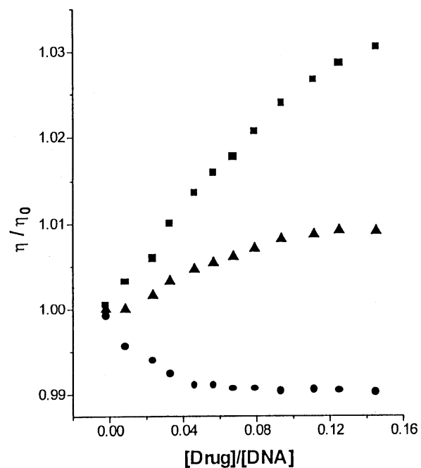
Figure 6. Plots of \eta/\eta_0 vs [\text{drug}]/[\text{DNA}] (buffer B) for [\text{Co}(\text{phen})_2(\text{phen-dione})]^{3+} ( \blacktriangle ), [\text{Co}(\text{phen})_3]^{2+} ( \bullet ) and [\text{Co}(\text{phen})_2(\text{dppz})]^{2+} ( \blacksquare ).
