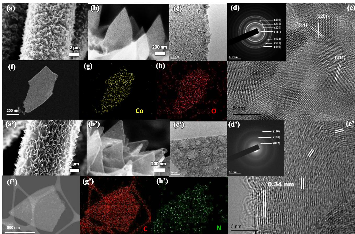
Fig. 2 (a-b) SEM images, (c) TEM image, (d) SAED pattern, (e) HRTEM image, (f) HAADF-STEM image, (g-h) EDX mapping result of \text{Co}_3\text{O}_4 nanosheets deposited on CC. (a'-b') SEM images, (c') TEM image, (d') SAED pattern, (e') HRTEM image, (f') HAADF-STEM image, (g'-h') EDX mapping result of porous N-doped carbon nanosheets deposited on CC.
