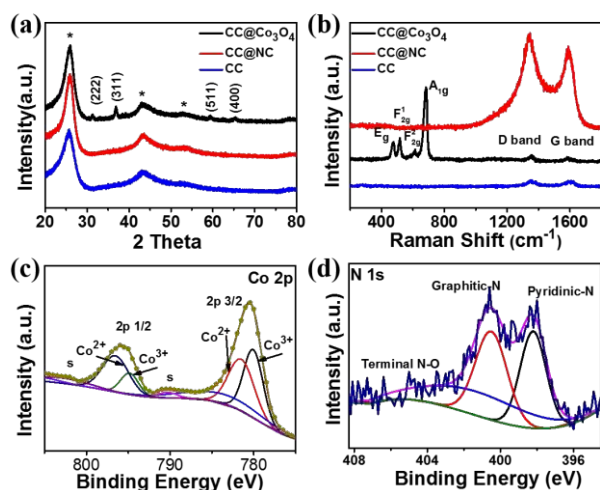
Fig. 3 (a) XRD and (b) Raman results of CC, CC@Co 3 O 4 and CC@NC. XPS spectra of (c) Co 2p in CC@Co 3 O 4 and (d) N 1s in CC@NC.
