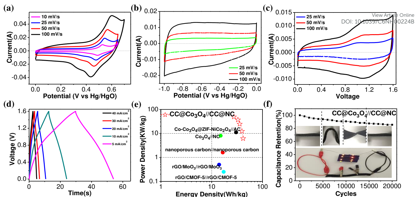
Fig. 4 CV curves of (a) CC@Co 3 O 4 , (b) CC@NC, (c) CC@Co 3 O 4 //CC@NC; (d) charge-discharge curves, (e) Ragone plots, and (f) Cycling test result of the asymmetric supercapacitor with PVA-KOH gel electrolyte. Insert in (f) shows digital images of the flat, bending, and twisting states of the cell during cycling test (upper) and a demo that three full cells (each size of 1*2.5*0.08 cm 3 ) can light up 8 orange LEDs.
