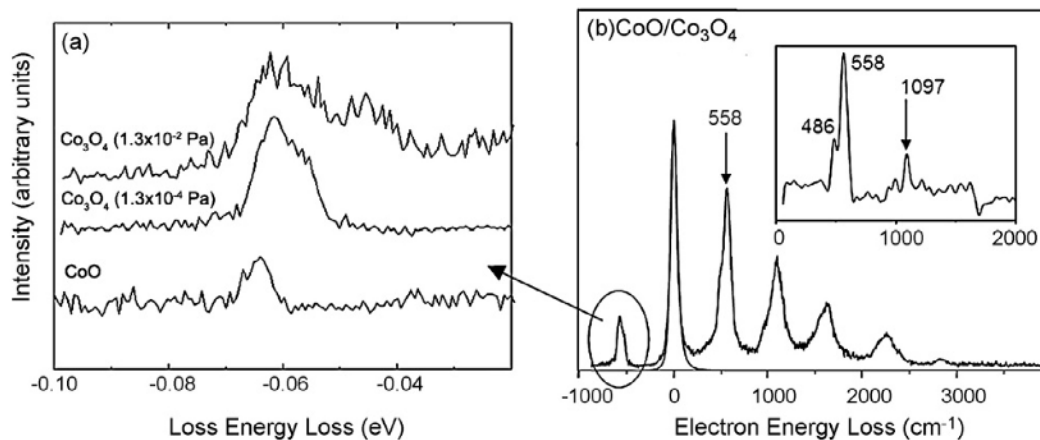
Figure 7. HREELS of (a) cobalt oxide series showing the changes in the energy gain peak, and (b) the full spectrum of the CoO/Co 3 O 4 epitaxial layer showing the electron scattering from Fuchs-Kliewer phonon modes. The inset in part (b) shows the deconvolution of the multiple scattering events to yield the single-loss data. The primary scattering beam energy is 3.77 eV.
