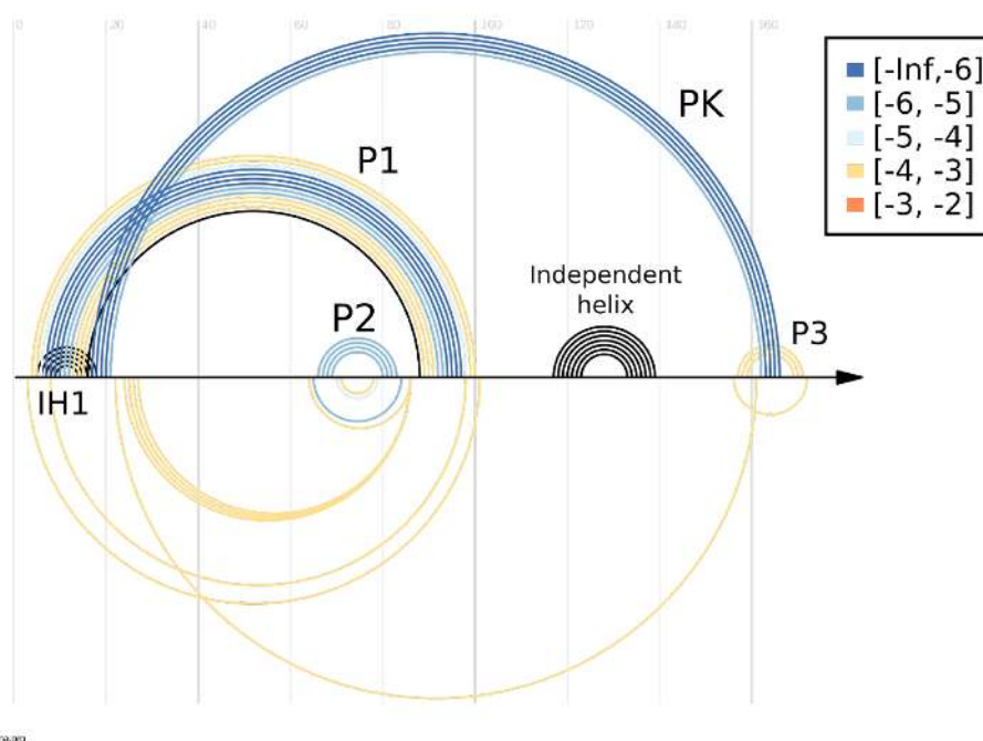
Figure 12. Sensitivity-specificity plot for the comparative COBOLD predictions for the ZTP riboswitch for a P -value threshold of 10^{-3} . The top of this figure shows the known RNA structure features. All non-black features correspond the features that have been correctly predicted by COBOLD. These are colored depending on the statistical significance of the corresponding predicted helix. Only the independent helix is missing from the COBOLD predictions. The bottom part of the figure shows only a few predicted base-pairs that are not part of the known RNA structure. The bottom part of the figure thus illustrates the high specificity of COBOLD (which would be perfect if no features were shown below the line), whereas the top part of the figure thus conveniently summarises the high sensitivity of the COBOLD predictions (hence the name sensitivity-specificity plot for this kind of figure). Overall, COBOLD thus readily recovers the experimentally confirmed RNA structure features that matter for the co-transcriptional folding pathway of the ZTP-riboswitch with high sensitivity and specificity.
