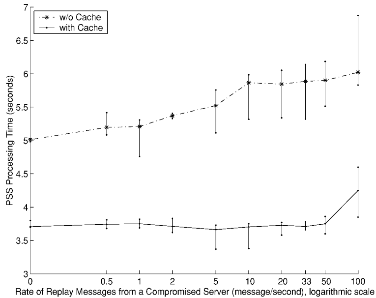
Fig. 8. Performance of proactive secret-sharing under the simulated denial-of-service attack from a compromised server: with cache versus without cache.
