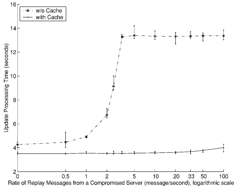
Fig. 7. Performance of Update processing under the simulated denial-of-service attack from a compromised server: with cache versus without cache.
