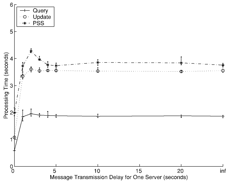
Fig. 9. Performance of COCA versus message delay for one server. Message delay of inf indicates the case where this one server is unavailable.
