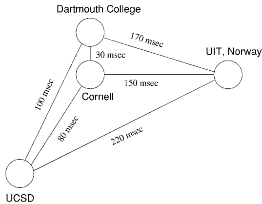
Fig. 3. Deployment of COCA over the Internet with message delays between servers.
