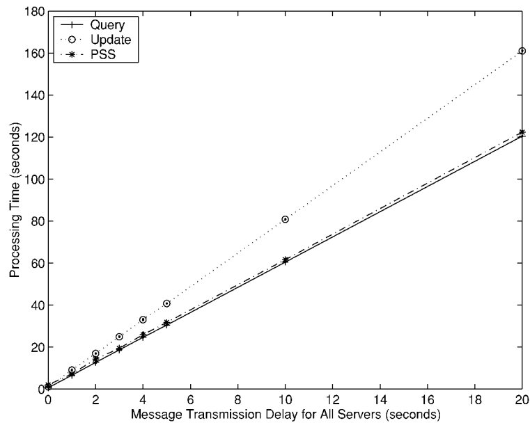
Fig. 10. Performance of COCA versus message delay for all servers.
