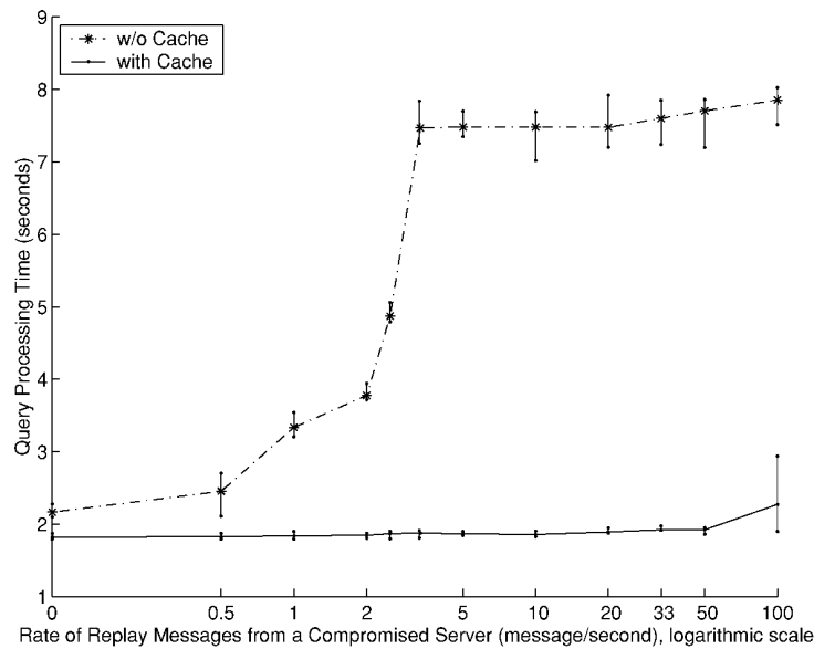
Fig. 6. Performance of Query processing under the simulated denial-of-service attack from a compromised server: with cache versus without cache.
