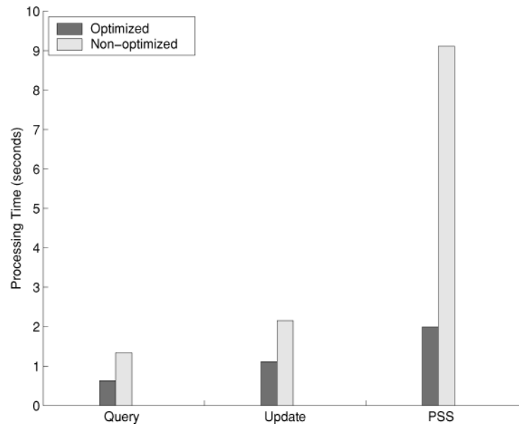
Fig. 2. Effectiveness of optimization in Query, Update, and proactive secret-sharing when assumptions N1 and N2 hold.
