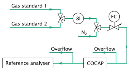
Figure 5. Setup used to determine a calibration curve for the CO 2 sensor. FC is a mass flow controller. The 8L buffer volume was flushed with either of two gas standards differing in CO 2 content, providing a slowly changing CO 2 dry air mole fraction. The second three-way valve is used to deliver nitrogen with zero CO 2 at the beginning and the end of each experiment.
