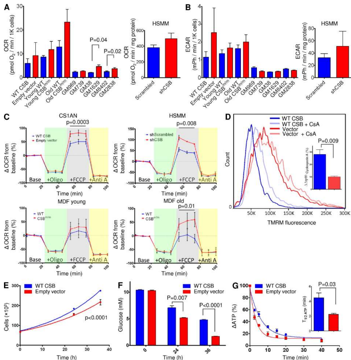
Figure 3. CSB deficiency increases cellular metabolism. (A and B) Oxygen consumption rates (OCRd; A) and extracellular acidification rates (ECARd; B) were increased in CSB-deficient cells. CS1AN: CSB patient cell line expressing an empty vector or a vector containing WT CSB. HSM: HSMs expressing scrambled shRNA or shRNA targeted to CSB. MDF: MDFs isolated from young and old CSB m/m mice. Primary CSB patient fibroblasts (GM739, GM1629, and GM2838) and healthy age-/gender-matched controls (GM969, GM38, and GM 8402) are shown. Blue are cells expressing WT CSB. Red are CSB-deficient cells ( n = 3-7 ; data are represented as mean \pm SEM). (C) FCCP-uncoupled respiration was measured by sequential addition of oligomycin (green background), FCCP (gray background), and antimycin A (yellow background; n = 3-7 ; data are represented as mean \pm SEM). (D) Mitochondrial membrane potential in CS1AN cells measured by 20 nM TMRM staining and flow cytometry and its responsiveness to treatment with cyclosporin A (CsA). Inset: quantification of the response to cyclosporin A ( n = 3 ; data are represented as mean \pm SEM). (E) Growth curve of CS1AN cells expressing either an empty vector or WT CSB. ( n = 3 ; data are represented as mean \pm SEM). (F) Glucose concentration was measured in the media of CS1AN cells expressing WT CSB or an empty vector ( n = 3 ; data are represented as mean \pm SEM). (G) ATP consumption of CS1AN cells expressing WT CSB or an empty vector after inhibition of ATP production with 100 mM 2-deoxyglucose and 1 \mu M oligomycin. Inset: half-life of ATP ( n = 3 ; data are represented as mean \pm SEM).
