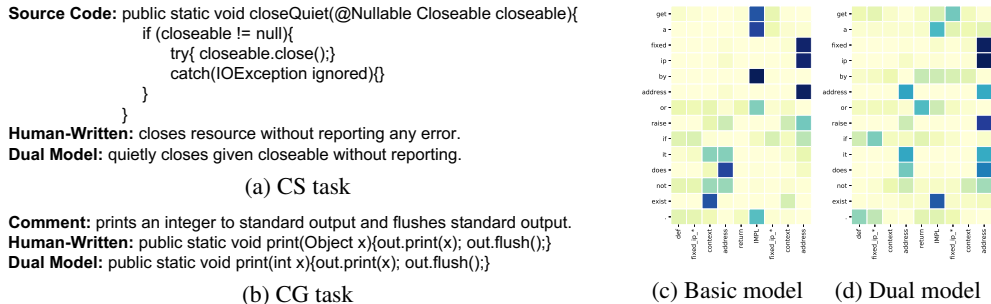
Figure 2: Qualitative analysis of our dual model. (a) Example of the generated comment given Java methods. (b) Example of the generated Java methods given natural language description. (c) Attention weights of basic model on CS task. (d) Attention weights of dual model on CS task.
