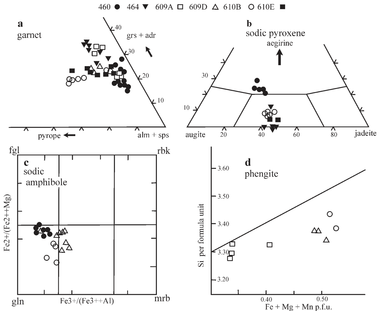
Figure 10. Garnet, sodic pyroxene, sodic amphibole and phengite compositions from the eclogites in the Çetmi melange. Abbreviations: alm, almandine; adr, andradite; fgl, ferroglaucophane; gln, glaucophane; grs, grossular; mrb, magnesioriebeckite; rbk, riebeckite; sps, spessartine.
