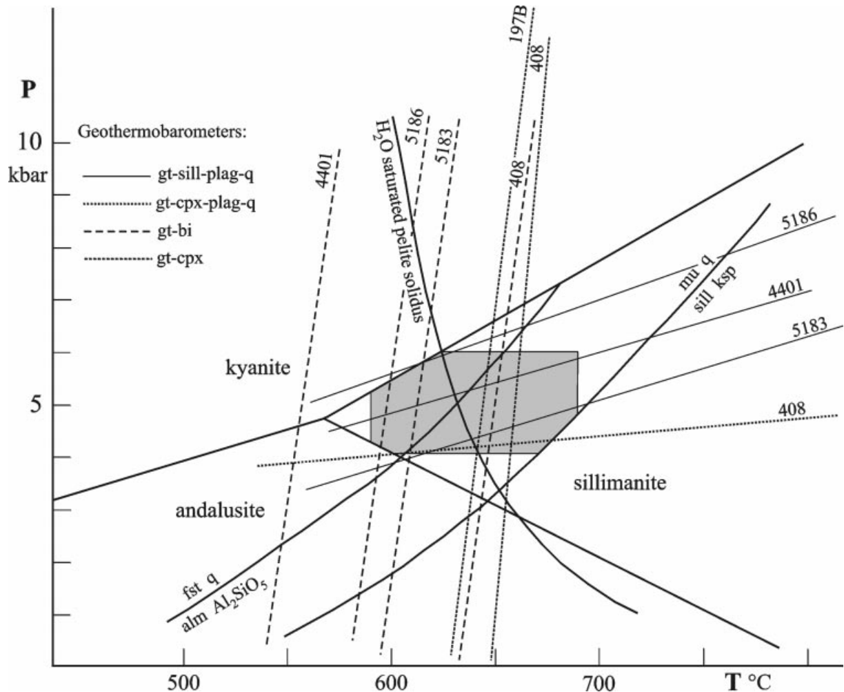
Figure 8. Pressure–temperature diagram illustrating the estimated P – T conditions of metamorphism and the relevant equilibria in the Kazdağ Massif. The end-member reactions are from the THERMOCALC program of Holland & Powell (1990). For the various geothermobarometers see the text. Abbreviations: alm, almandine; bi, biotite; cpx, clinopyroxene; fst, ferrostauroilite; gt, garnet; ksp, K-feldspar; mu, muscovite; plag, plagioclase; q, quartz; sill, sillimanite.
