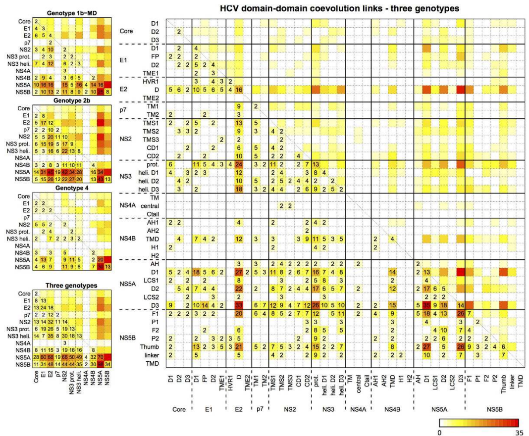
Figure 6. Matrices describing HCV coevolving proteins and domains. Left: The four matrices describe the analysis of protein-protein coevolution links for genotypes 1b-MD, 2b and 4 (top), and for the three genotypes confounded (bottom). Numbers in the matrices count coevolving residues (hits) belonging to clusters predicted by BIS 2 analysis (see Methods). These numbers are intended to be indicators of the “amount of evidence for a coevolution link”. The diagonal (from the top left to the bottom right) of each matrix corresponds to internal coevolution links between residues in the same protein. The color scale used in each matrix corresponds to the range of the coevolving links computed for the matrix and it goes from red (maximum value for the matrix) to white (0). Note that the thickness of the edges in Fig. 5A corresponds to the entries of the matrix for the three genotypes (bottom). Right: The large matrix describes the analysis of domain-domain coevolution links, for the three genotypes 1b-MD, 2b and 4. It is the detailed domain-domain analysis of the protein-protein matrix shown on the top left. Thick black lines are drawn to delimit different proteins, while dotted lines delimit their domains. Detailed analyses for genotypes 1b-MD, 2b and 4 are reported as Supplementary Figures 4–6. Note that the sum of the entries for two proteins does not correspond to the value of the corresponding protein-protein entry in the matrix at the bottom left. Take, for instance, the interaction NS2-NS4A. Cluster 28 of genotype 1b-MD has 1 hit in NS4A and 2 hits in NS2, located these latter in the two different domains TMS1, TMS2. In the matrix on the bottom left, the entry NS2-NS4A is 3 since a total of 3 hits identifies the NS2-NS4A interaction. On the other hand, the domain-domain matrix reports 2 hits for NS4A-NS2/TMS1 and 2 for NS4A-NS2/TMS2, with a sum of the domain entries equal 4.
