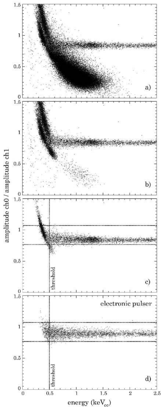
FIG. 10. Steps in data selection through the UC analysis pipeline: a) All data including microphonics-intensive periods of LN2 Dewar filling. b) Following removal of LN2 transfer periods and ensuing 10 minutes (boiling in the Dewar lasts a few minutes). No correlated excess of events is observed to extend beyond this 10 min cut. c) Following application of cuts intended to remove anomalous electronic pulses (see text). The boundaries for a final cut using the CH0/CH1 amplitude method in [24] are shown as horizontal lines. These boundaries are selected to minimize the effect of this cut for both radiation-induced and pulser events, with the exception of a distinct family of residual microphononic events visible as a diagonal band in this panel. d) Fast electronic pulser events prior to any cuts (only the CH0/CH1 amplitude criterion is seen to minimally affect these).
