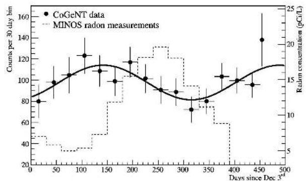
FIG. 29. Counts per 30 day bins from the 0.5-3.0 keV CoGeNT energy window (black dots) compared to the MINOS radon data at SUL (dashed), averaged over the period 2007-2011, exhibiting a peak on August 28th [44, 45]. The solid curve represents a sinusoidal fit to CoGeNT data. An analysis by the MINOS collaboration finds a three-sigma inconsistency between the phase of their measured seasonal modulation in radon concentration at SUL and CoGeNT data [26].
