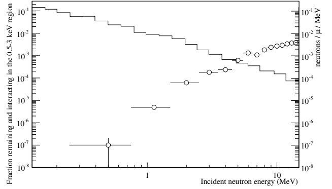
FIG. 26. Fraction of external ( \mu,n ) cavern neutrons giving rise to energy depositions in the 0.5-3.0 keVee energy window of the CoGeNT detector at SUL, as a function of incident neutron energy, derived from a Monte Carlo simulation (open circles). Also shown, using the right-hand scale, is the emission energy spectrum for these neutrons, taken from [43] (histogram).
