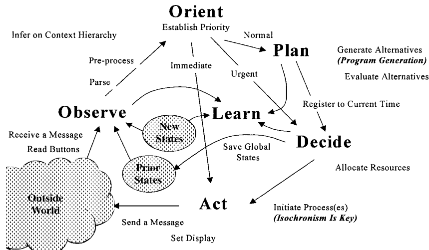
Figure 1. The cognition cycle.
