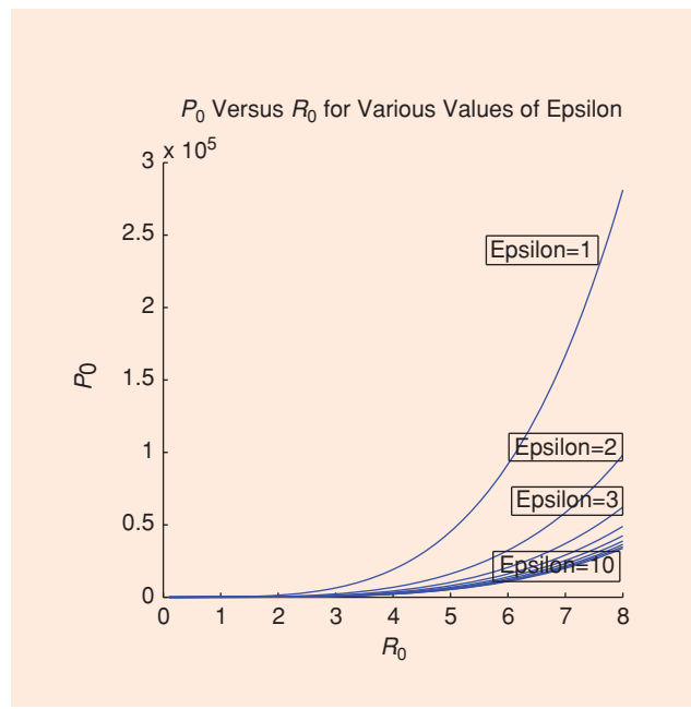
[FIG10] The relation between the BS power P_0 and the exclusive region radius R_0 according to (4) for \lambda = 1 , P = 1 , \sigma^2 = 1 , \beta = 0.1 , C_0 = 3 and \alpha = 3 .
