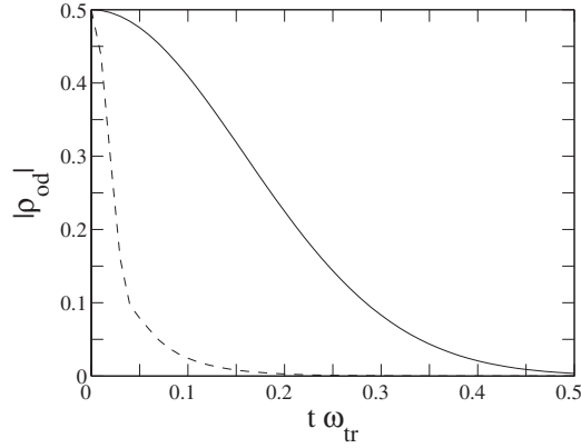
FIG. 9. Decay of the off-diagonal element at T=10 nK as a function of t\omega_{\text{tr}} . Dashed line shows the decay in the case of the thermal coherent occupation and the solid line shows the decay in the case of the thermal occupation.
