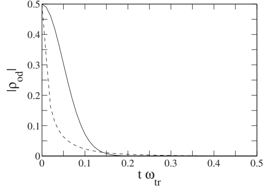
FIG. 10. Decay of the off-diagonal element for T=100 nK and thermal coherent occupation of the zero mode as a function of t\omega_{\text{tr}} . Dashed line shows the decay in the case of the thermal coherent occupation and the solid line shows the decay in the case of the thermal occupation.
