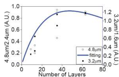
FIGURE 4. Sample dependence. Coherent control generated terahertz peak-peak amplitude for 4.8 and 3.2\ \mu\text{m} fundamental beam wavelengths, taken at different positions on various multilayer epitaxial graphene samples with different numbers of layers. The 4.8 and 3.2\ \mu\text{m} pump beams give different terahertz peak amplitudes, so the data are normalized so the two different pump beams yield the same peak signal on the 63 layer sample.
