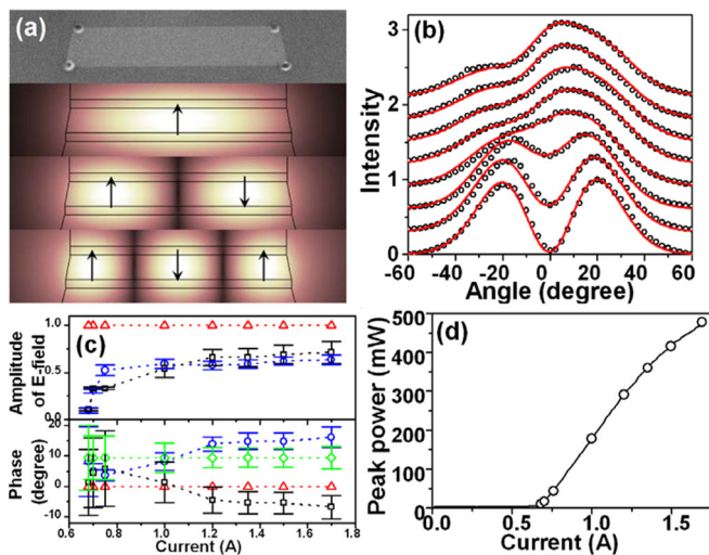
FIG. 2 (color online). (a) SEM image of the facet of a QCL with a 12- \mu\text{m} -wide active region, and simulations showing from top to bottom the electric field of TM 00 , TM 01 , and TM 02 modes for the device; the arrows in the figure indicate the polarization of the field. (b) Measured far-field intensity distributions of the device (open circles) and their fits (solid lines) at driving currents of 1.7, 1.5, 1.35, 1.2, 1, 0.75, 0.70, and 0.68 A (from top to bottom). The curves are shifted vertically for clarity. (c) Electric-field amplitude (upper panel) and phase (lower panel) of the transverse modes used to fit the far-field data in (b). Open circles: TM 00 mode; open triangle: TM 01 mode; open squares: TM 02 mode; open diamonds: \phi_{TM00} + \phi_{TM02} - 2\phi_{TM01} . Dotted lines are used to guide the eyes. Error bars indicate the range of individual parameter changes that will lead to a root mean square deviation of 0.05 between the experimental data and the fits. (d) Light output versus current (LI) curve for the device. The LI curve is free of kinks, indicating a smooth growth of all the mode components. The dots indicate the operating conditions at which the near- and far-field measurements were performed.
