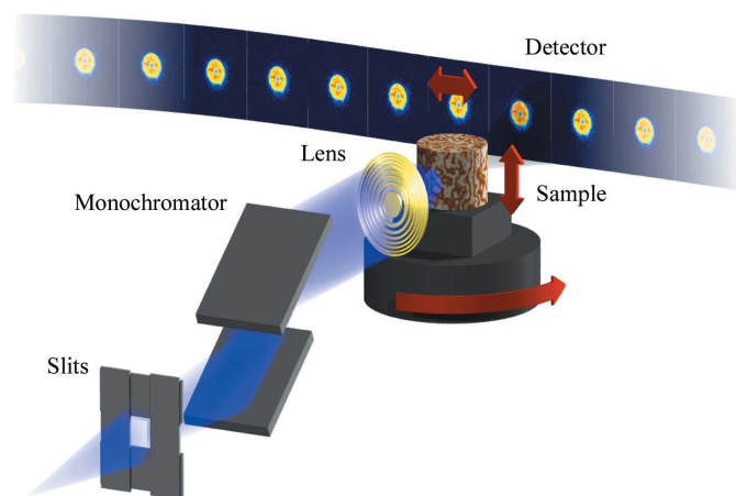
Figure 1 Schematic of a typical ptychography set-up. The X-ray beam generated by the insertion device is filtered spectrally with a monochromator, admitted through one or multiple beam-defining apertures, which act as a coherence filter as well, and focused on the sample. For each position of the sample in the beam, i.e. lateral displacement and rotation, the intensity of the scattered X-ray wave is measured in the far-field using a pixel array detector.
