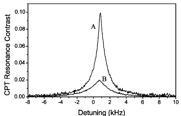
Fig. 2. CPT resonance for excitation on A, the D_1 transition and B, the D_2 transition with a resonant laser intensity of 160 \mu\text{W}/\text{cm}^2 .
