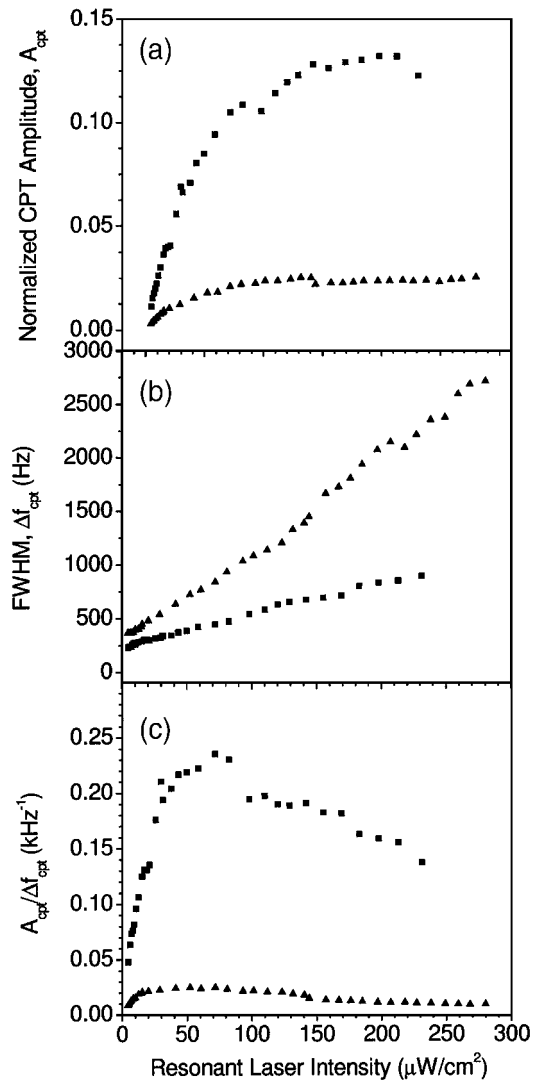
Fig. 3. CPT (a) amplitude, (b) width, and (c) quotient of both quantities, measured for excitation on the D_1 (squares) and the D_2 (triangles) transitions.
