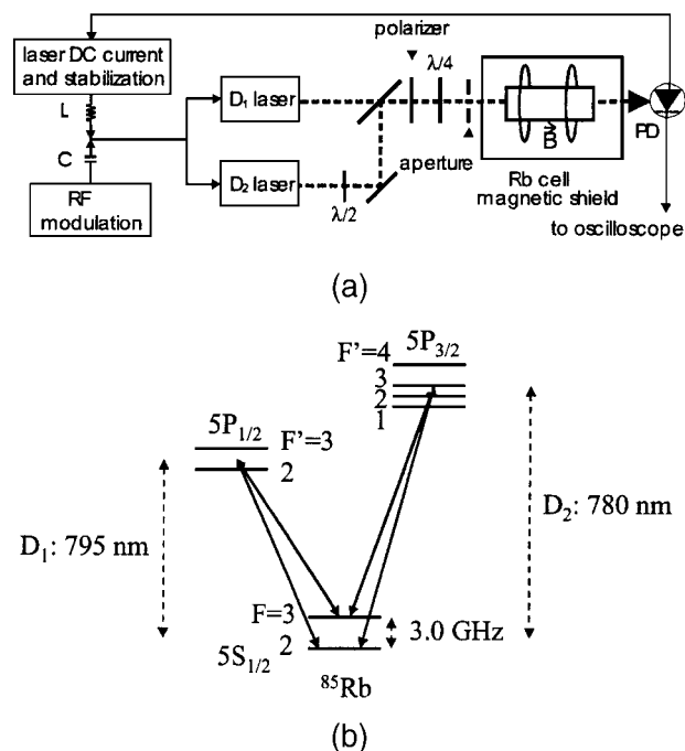
Fig. 1. Experimental setup for the comparison of the CPT resonances for excitation when the D_1 and the D_2 transitions are used.
