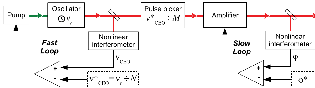
Figure 11 Scheme for active CEP stabilization; v_{CEO}^* and \phi^* are the target values of v_{CEO} and \phi , respectively.
