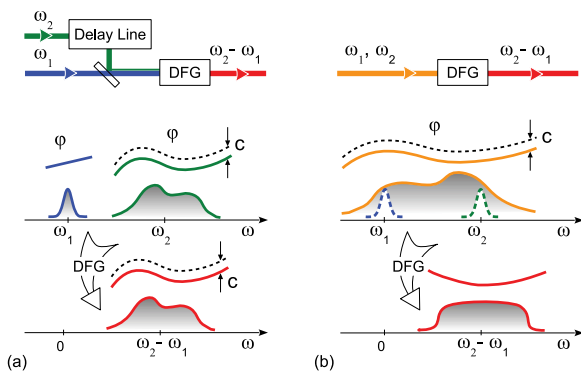
Figure 12 Comparison of (a) inter-pulse and (b) intra-pulse stabilization schemes. Lower panels show the evolution of both intensity and phase in the frequency domain; \phi is the absolute phase, c denotes fluctuations of the CEP.
