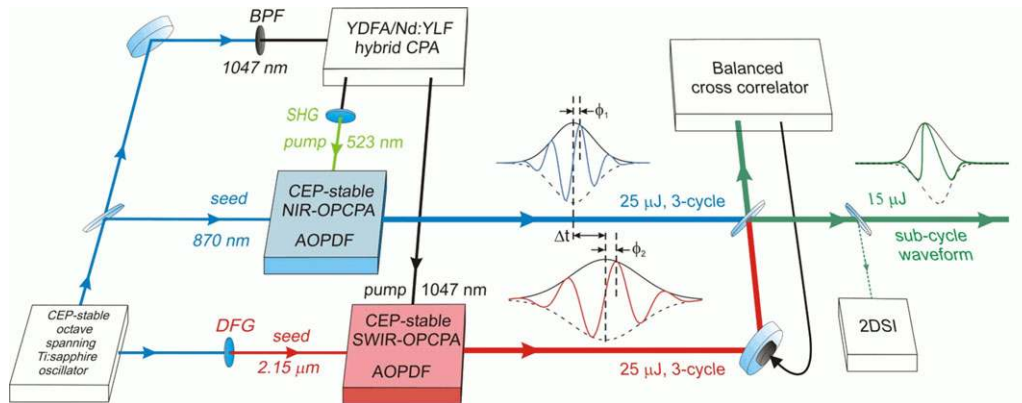
Figure 31 Scheme of the high-energy OPCPA waveform synthesizer from [66]. BPF: bandpass filter; SHG: second-harmonic generation crystal; DFG: intrapulse difference-frequency generation module; AOPDF: acousto-optic programmable dispersive filter.
