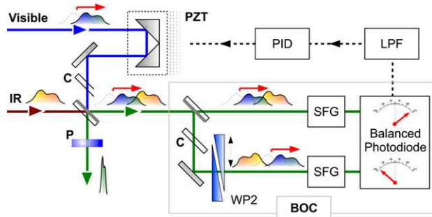
Figure 35 Schematic of the synthesizer and the BOC. PZT: piezoelectric actuator; WP2: \text{CaF}_2 wedge pair for delay tuning; P: 2 mm thick \text{CaF}_2 plate; C: compensation plates; LPF: electronic low-pass filter; SFG: sum-frequency generation; PID: proportional–integral–derivative controller.
