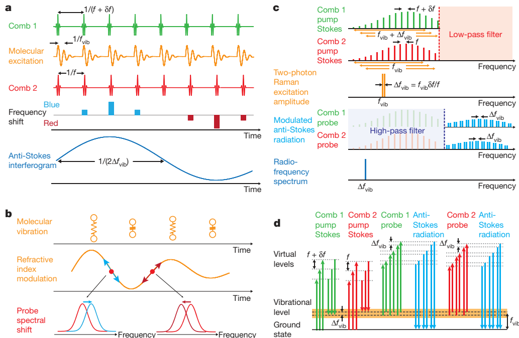
Figure 1 | Principle of dual-comb CARS. \Delta f_{\text{vib}} stands for f_{\text{vib}}\delta f/f . a , Time-domain representation in the limit of a molecular decoherence time that is shorter than the time interval between two laser pulses. The train of pulses of laser frequency comb 1 periodically excites the molecular vibration, which is probed by the pulses of laser frequency comb 2 with a linearly increasing time delay. The resulting filtered anti-Stokes radiation provides the interferogram. The two combs have a symmetric function. In the figure, only the situation in which the delay between the pulses of comb 2 and those of comb 1 is positive is displayed. b , When the probe pulse is short compared with the molecular oscillation (impulsive stimulated Raman scattering), the refractive index
