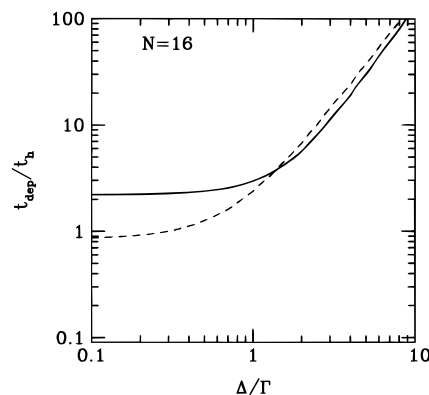
Figure 5. Depolarization time t_{\text{dep}} divided by the Förster hopping time t_{\text{h}} = \Gamma/2J^2 as a function of the ratio of disorder \Delta divided by the homogeneous line width \Gamma . In this figure results for a ring of N = 16 pigments are presented and \Gamma = J . The dashed curve is the result of the diffusion approximation, and the solid curve the exact exciton result. Disorder reduces the effect of coherent exciton dynamics.
