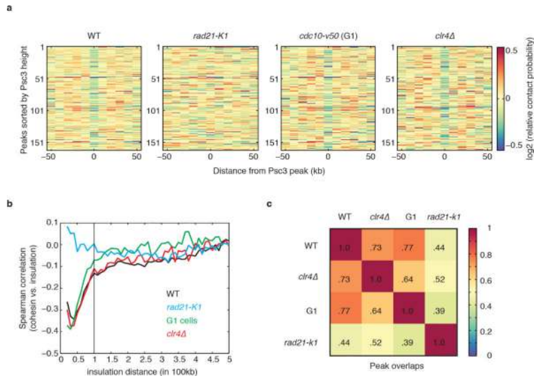
Extended Data Figure 7. Globule boundaries in wild type, rad21-K1 , G1 arrested and clr4Δ a , Insulation effect for all cohesin (Psc3) peaks. Relative contact probability was averaged over 20-50kb at each Psc3 peak region (-50kb to +50kb region) and sorted by Psc3 peak height. Insulation effect at Psc3 peaks in wild type, G1, and clr4Δ holds genome-wide, and not only at a small subset of peaks. b , The correlation between Psc3 and relative contact probability R_j(s) profile at a given distance s . The negative correlations hold up to 100kb in wild type, G1 arrested cells and clr4Δ . Psc3 enrichment and the relative contact probability profile in rad21-K1 do not show an appreciable correlation at any distance. c , The fraction of overlapping boundaries ( \pm 1 bin) for each Hi-C dataset is shown. Boundaries in clr4Δ and G1 arrested cells show high overlap with wild type boundaries. The top 100 strongest boundaries from each dataset were examined for comparison.
