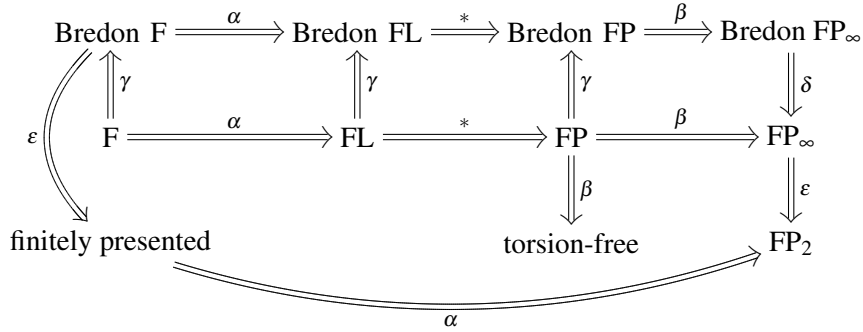
FIGURE 1. Connections between cohomological finiteness conditions
