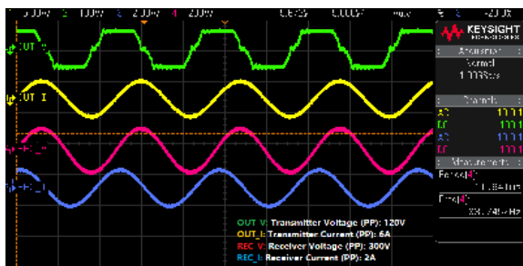
(a) Experimental waveforms of resonant circuit when angular offset is 0 in novel transmitter coil case
