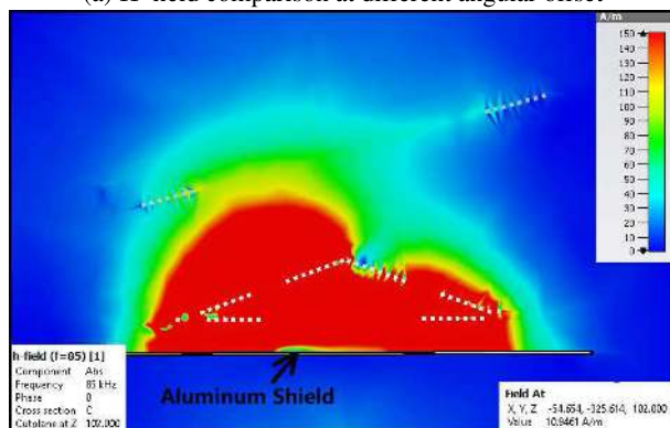
(b) Aluminum Shielding at 15 angular offset
