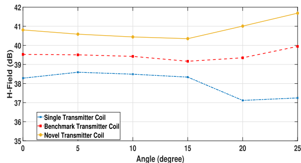
(a) H -field comparison at different angular offset
