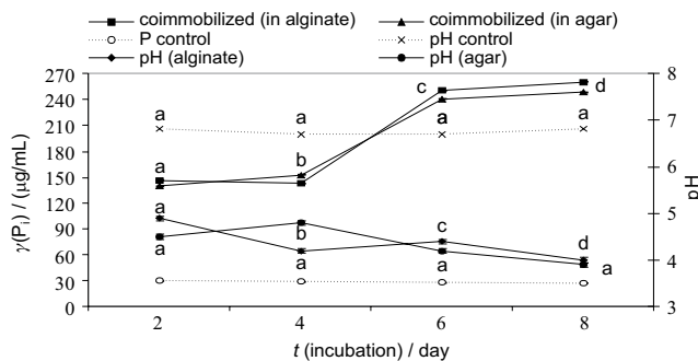
Fig. 2. Changes in pH and P concentrations in PVK broth by alginate or agar encapsulated bacterial isolates, a) B. megaterium , b) A. lipoferum 137, and c) coimmobilization. Points on each curve marked with a different letter differ significantly at P \leq 0.05 in one-way ANOVA. Bars represent the standard error (s.e.). When the s.e. bar is absent, the s.e. is smaller than the symbol used
