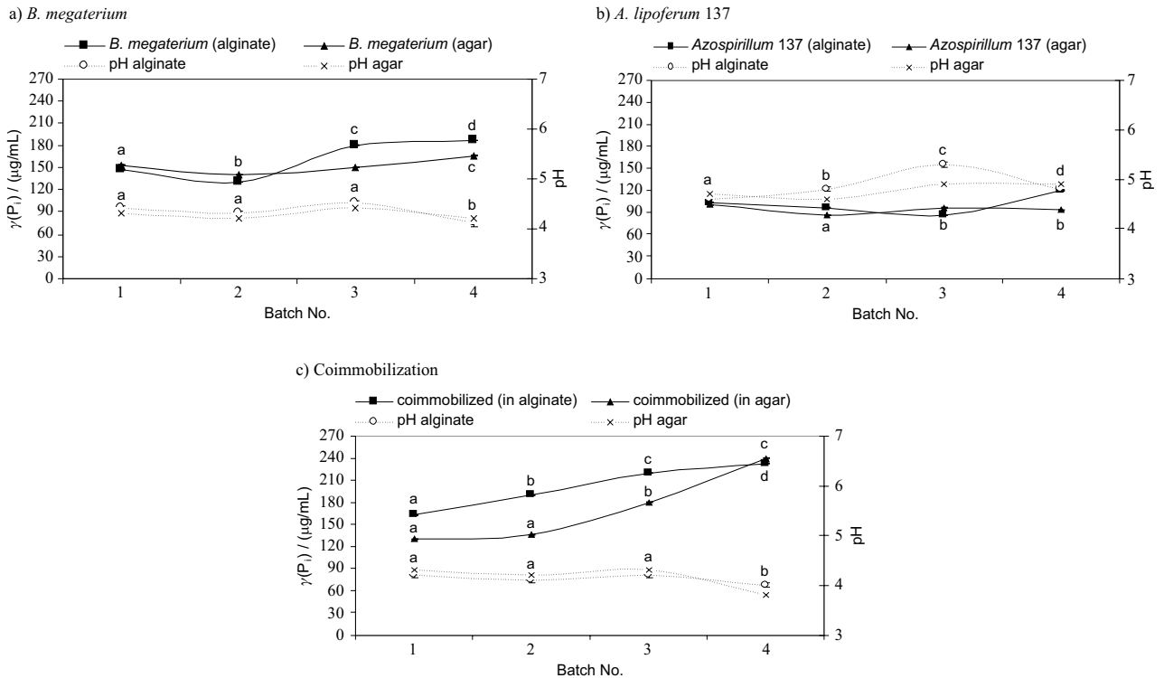
Fig. 3. Reusability of alginate or agar immobilized bacteria, a) B. megaterium , b) A. lipoferum 137, and c) coimmobilization for P-solubilization. Points on each curve marked with a different letter differ significantly at P \leq 0.05 in one-way ANOVA. Bars represent the standard error (s.e.). When the s.e. bar is absent, the s.e. is smaller than the symbol used
