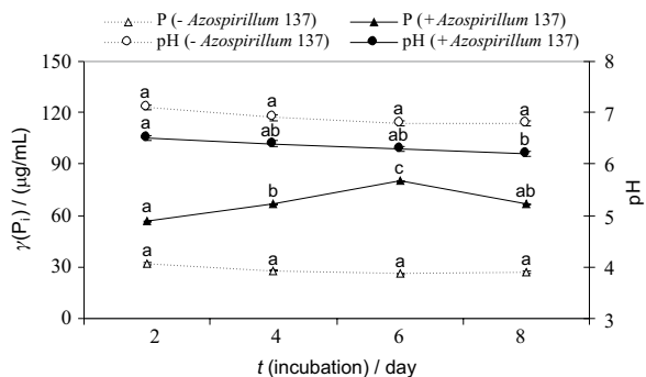
Fig. 1. Changes in pH and P concentrations in PVK broth in presence (+) or absence (-) of different bacterial isolates, a) P. fluorescens , b) B. megaterium , c) A. lipoferum 137, and d) A. lipoferum Z1. Points on each curve marked with a different letter differ significantly at P \leq 0.05 in one-way ANOVA. Bars represent the standard error (s.e.). When the s.e. bar is absent, the s.e. is smaller than the symbol used
