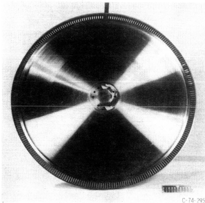
Figure 7. - Test rotor.
