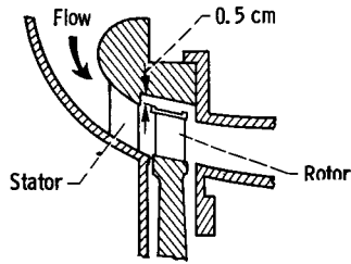
a) Original tip clearance configuration.
