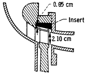
(b) Reduced tip clearance configuration.
