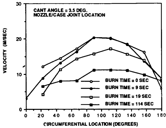
Fig 12. Circumferential Velocity Distribution
