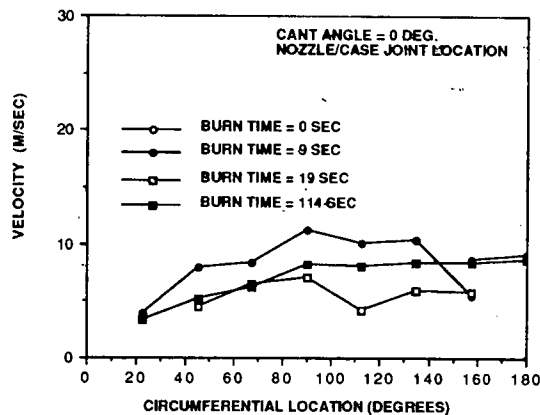
Fig 11. Circumferential Velocity Distribution
