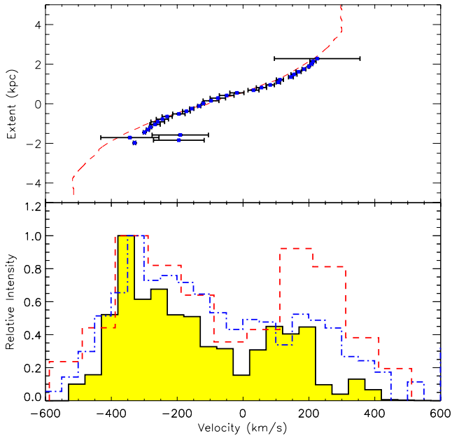
Figure 12. The Pa \alpha velocity profile along with a reconstructed spectrum. The reconstructed spectrum of the Pa \alpha bears a remarkable resemblance to those of the atomic (blue dot-dashed line) and molecular (red dashed line) line profiles. The Pa \alpha profile shows an asymmetry with more pronounced blue peak similar to that of the [O I] suggesting that they trace similar gas distributions. Note that all three show a double-peaked structure with a similar separation indicating that the CO and [O I] share the same velocity structure as the Pa \alpha .
