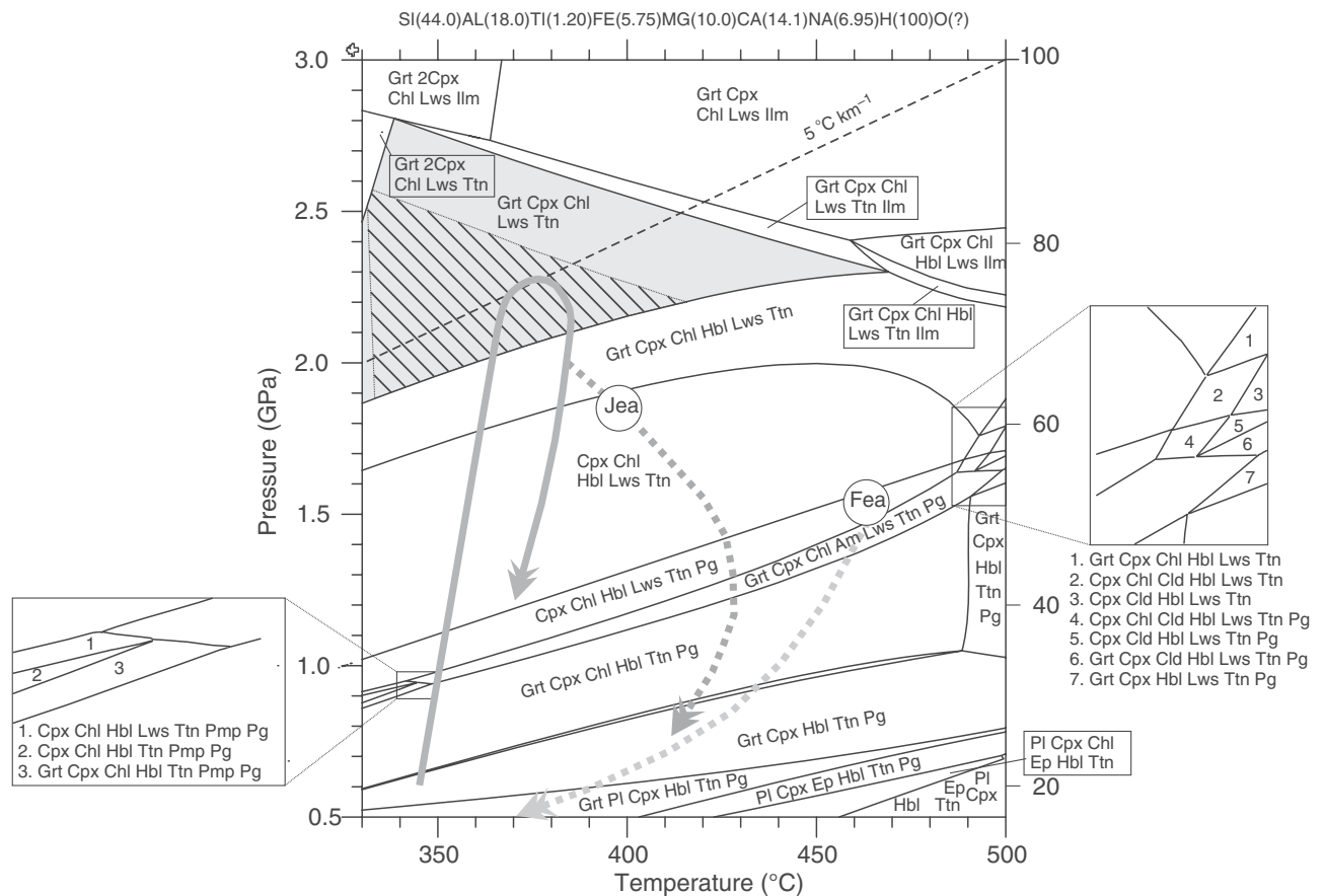
Fig. 7. Isochemical P - T phase diagram showing the stability fields for mineral assemblages in sample COR-1, calculated using Theriak-Domino. See text for discussion. Hatched area marks overlapping P - T conditions for peak assemblages in all three bulk compositions. Note that in the upper left corner are two small fields with two coexisting clinopyroxenes. A tentative P - T path of the Défilé du Lancône lawsonite eclogite based on textural observations and thermodynamic modelling is shown (solid hairpin arrow). Alternative retrograde P - T paths are taken from Fournier et al. , 1991 (Fea) and Jolivet et al. , 1998 (Jea).
