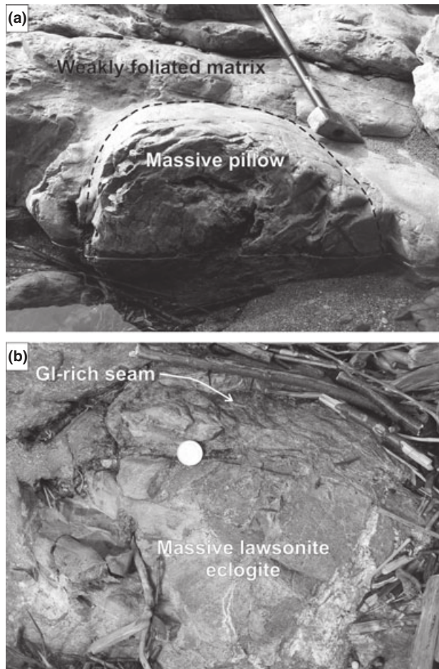
Fig. 3. Eclogitized pillow lava along the riverbed of Défilé du Lancône. (a) A well-preserved pillow with internal drain-out, convex upward cavity. Notice that the pillows have blue outer margins due to the superimposed blueschist facies metamorphism. (b) Details of a massive eclogitized pillow with a thin seam of glaucophanite.
