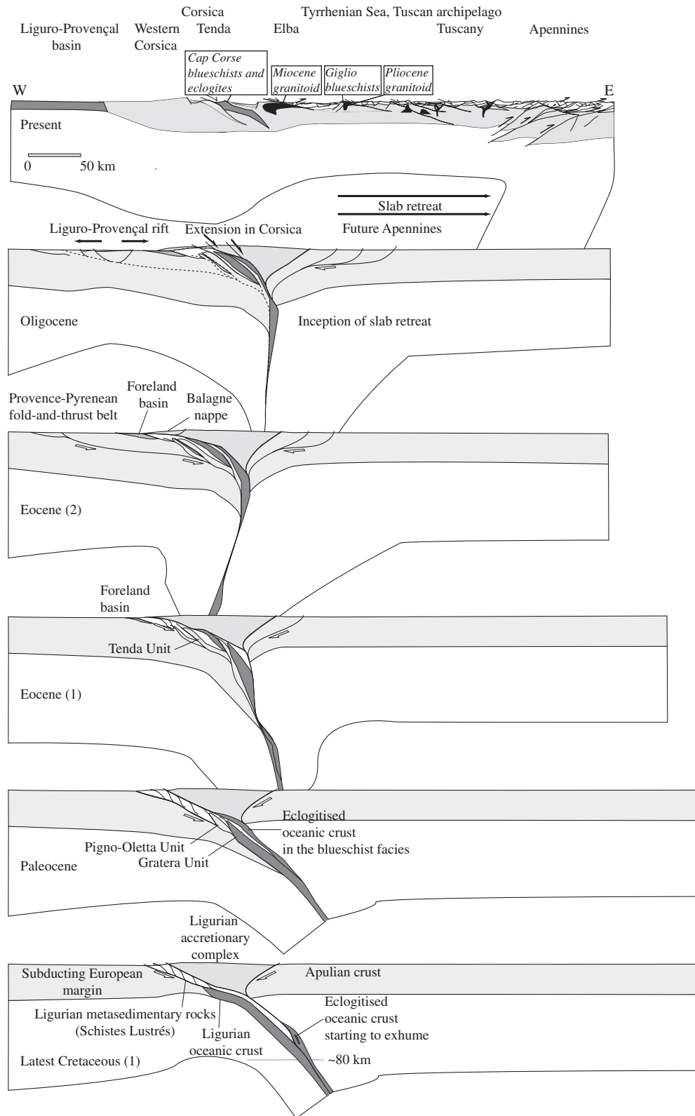
Fig. 10. Model of tectonic evolution of the Alpine LTHP metamorphic complexes Corsica (modified from Jolivet et al. , 1998), where the new P - T data from lawsonite eclogites in Défilé du Lancône have been incorporated. See text for discussion and details.
