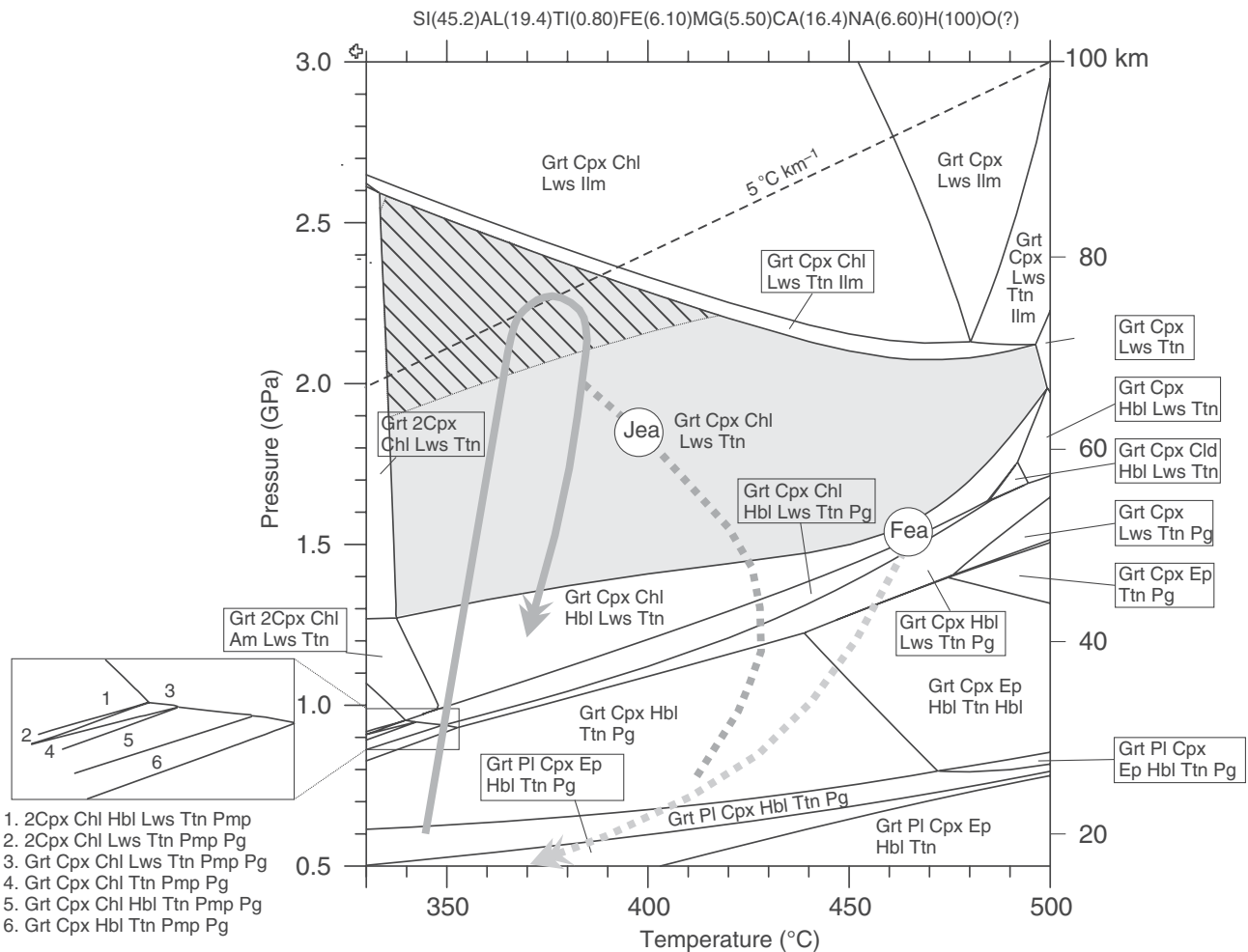
Fig. 8. Isochemical P – T phase diagram showing the stability fields for mineral assemblages in sample COR-4 matrix, calculated using Theriak–Domino. See text for discussion. Note that at 0.9–2.6 GPa and < 340 °C two coexisting clinopyroxenes can be stable.
