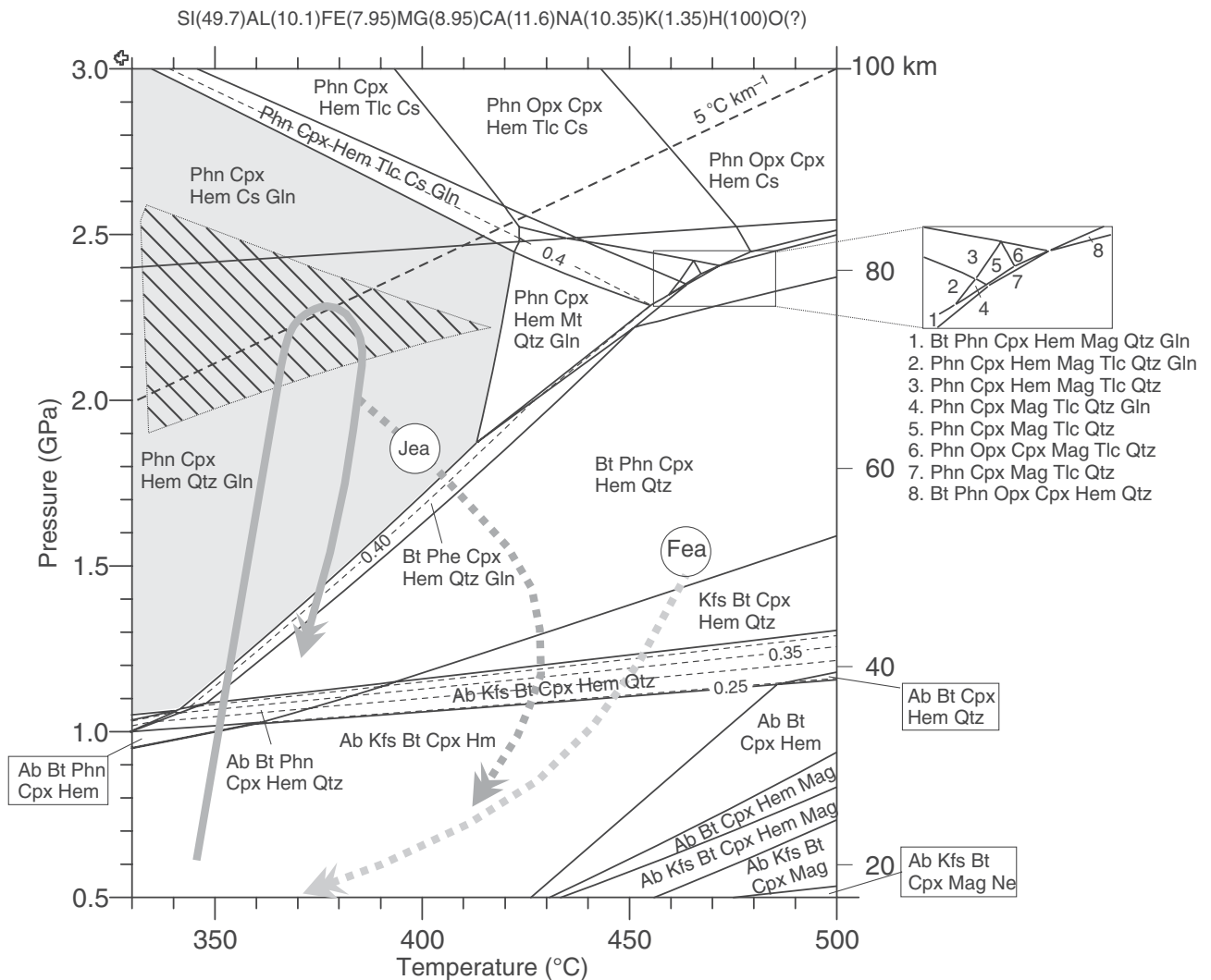
Fig. 9. Isochemical P - T phase diagram showing the stability fields for mineral assemblages in omphacite-rich veins, sample COR-4, using Theriak-Domino. Contours for jadeite content of clinopyroxene are shown as stippled lines. See text for discussion.
