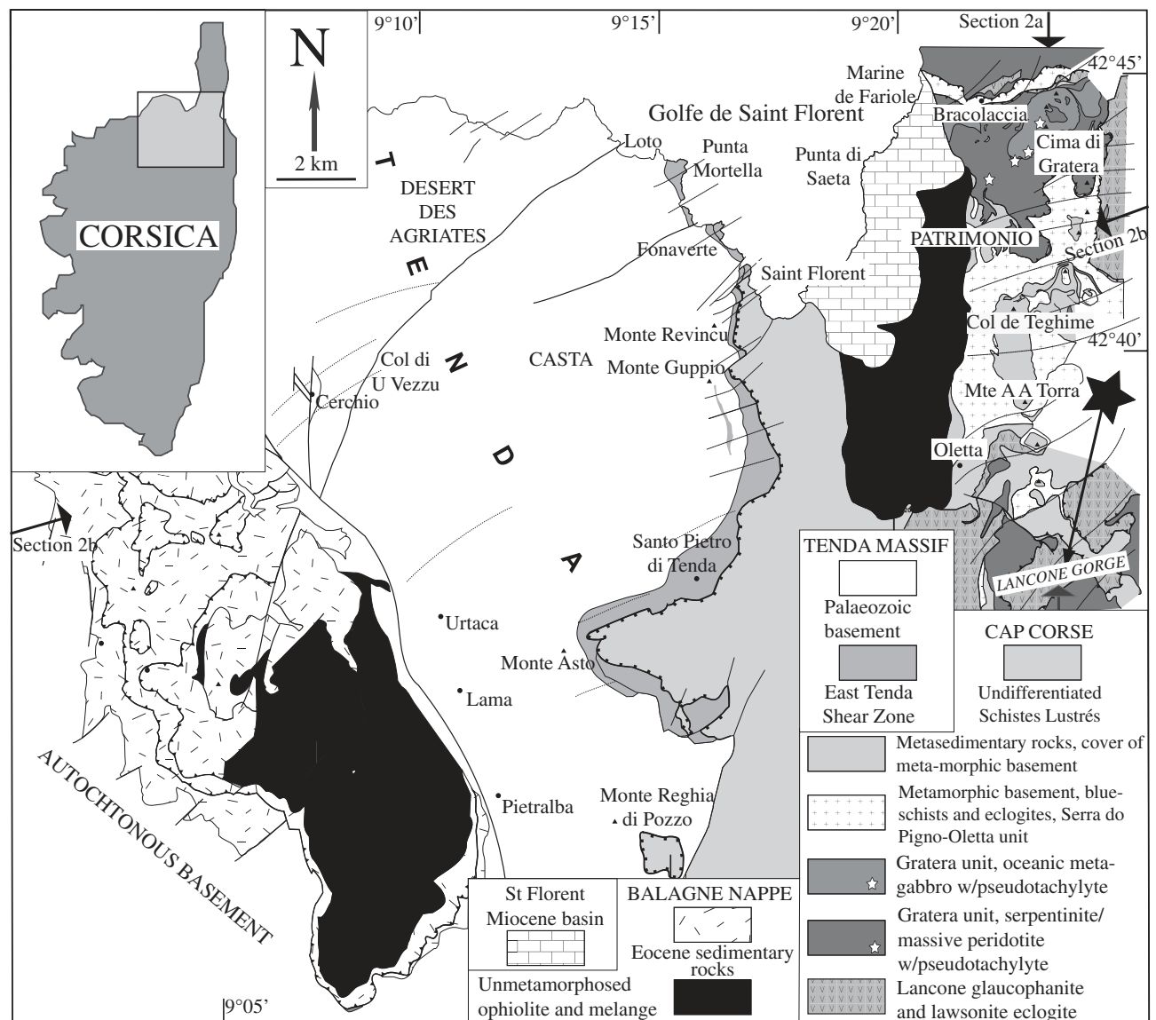
Fig. 1. Geological map of northern Corsica (see inset map for location) showing the main Alpine tectonic units and location of the new lawsonite eclogite locality in Défilé du Lancône (marked with star). Notice the location of subduction-related pseudotachylytes north of Patrimonio.
