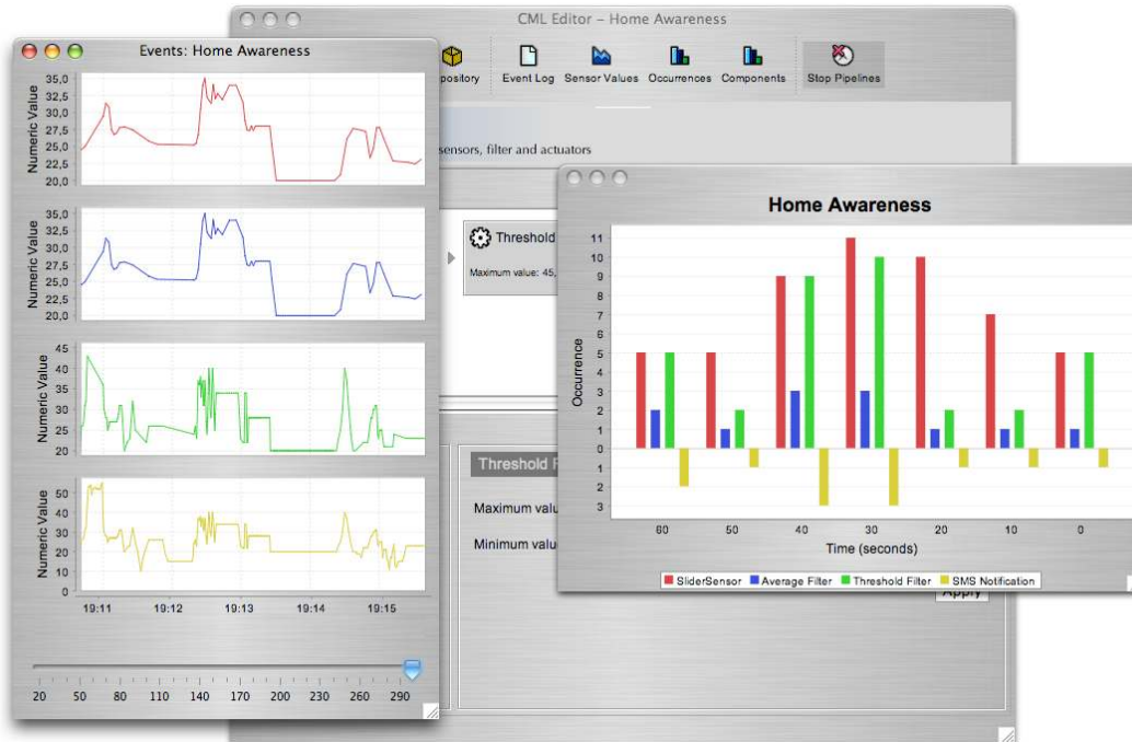
Figure 5. Real-Time Visualisation GUI (with time plot visualization, and overview of the pipeline events).
