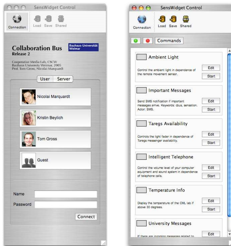
Figure 2. Login GUI and Control GUI.
