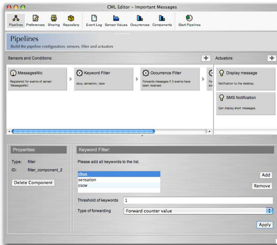
Figure 3. Editor GUI.
