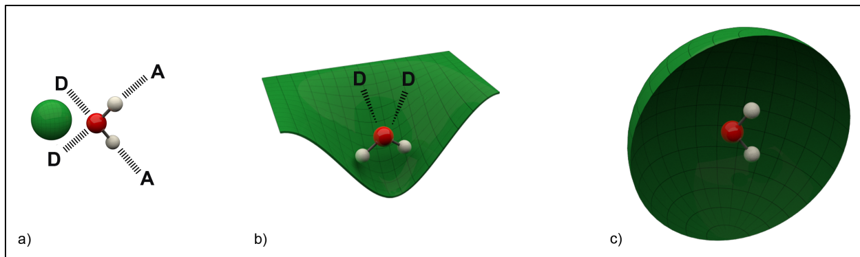
Figure 1: Illustration of how gross shape influences solute solvation: a) and c) are the two extremes of solvation: a) small convex solutes barely disrupt HBinding between waters and a solvation shell water can accept (A) and donate (D) four HBs. In contrast, an isolated molecule of water (c) cannot form any HBs with other waters. b) The intermediate case of solvating concavity, where any bound water only forms a limited number of HBs.
