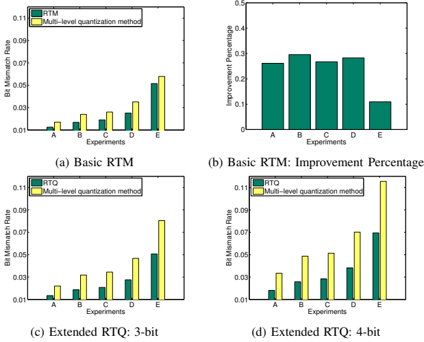
Fig. 4. Bit mismatch rate under various experimental scenarios.
