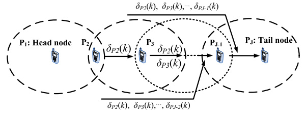
Fig. 8. Illustration of chain-based group key extraction protocol
