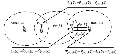
Fig. 5. Illustration of relay node assisted collaborative key extraction.
