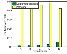
Fig. 3. Bit mismatch rate for legitimate devices and attacker under different scenarios.
