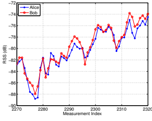
Fig. 1. Segments of RSS measurements from a pair of mobile devices in park.
