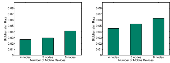
(a) A (park, with pedestrian) (b) B (park, without pedestrian) Fig. 10. Performance of chain-based group key extraction.
