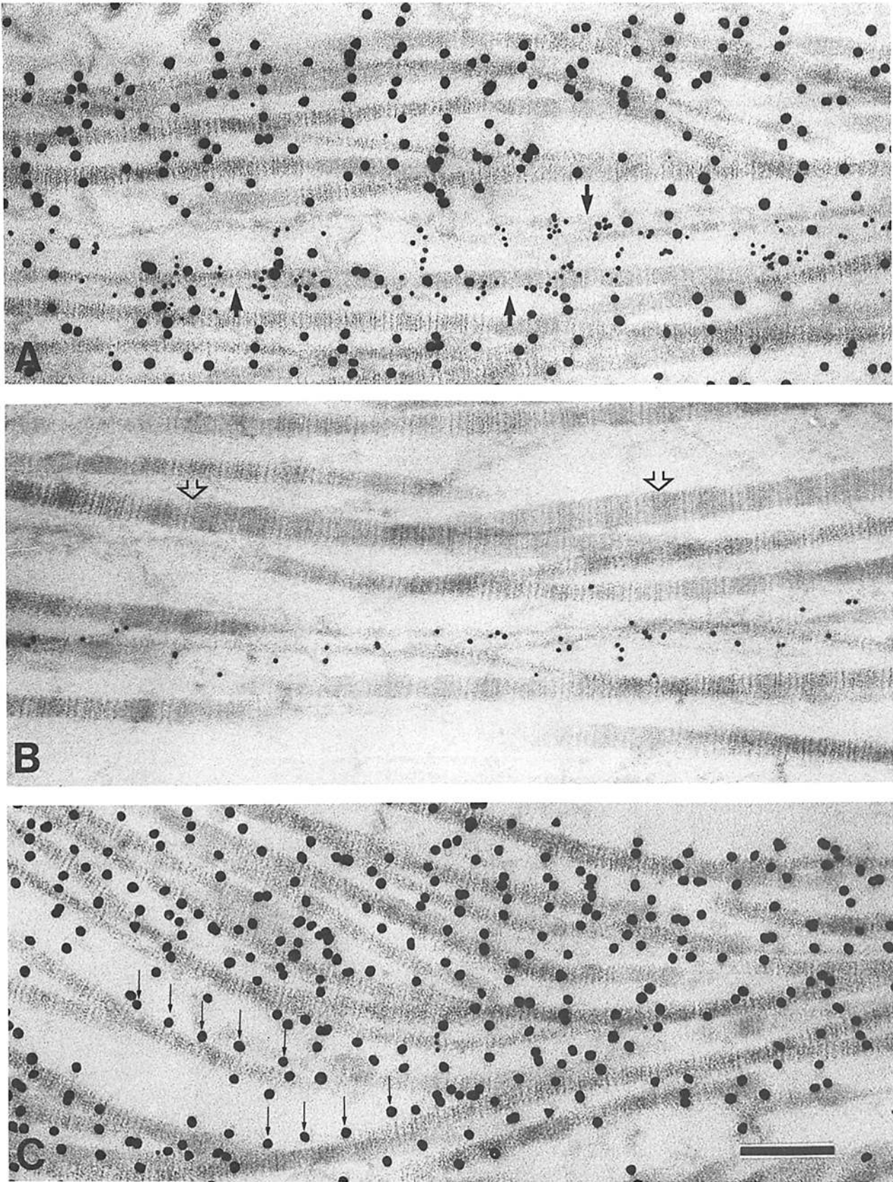
Figure 2. Colocalization of collagen types I and V in the lathyritic cornea pretreated at 4°C. Sections from lathyritic corneas were incubated in PBS for 15 h at 4°C, a condition where fibril structure is partially disrupted, fixed in paraformaldehyde, and incubated simultaneously with two different monoclonal antibodies coupled directly to either 5 or 10 nm colloidal gold particles. A was incubated with monoclonal antibodies against type I collagen coupled to 10 nm gold and against type V collagen coupled to 5 nm gold particles; B was incubated
