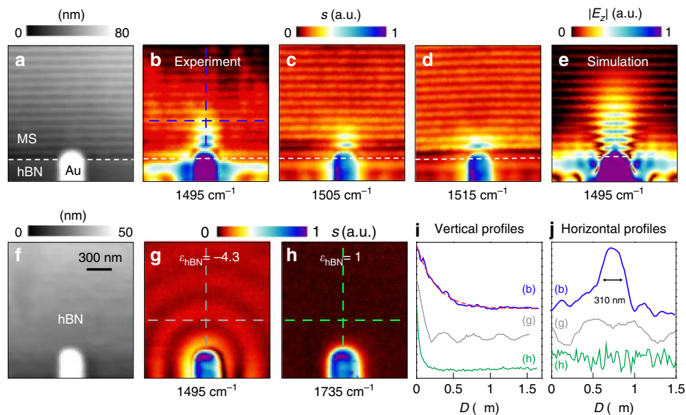
Fig. 4 Real-space imaging of polariton canalization in a hBN metasurface. a Topography of the sample. b–d Experimental near-field distribution of antenna-launched elliptical polaritons on the metasurface at three different frequencies. White dashed lines mark the boundary of the metasurface. e Simulated near-field distribution of the antenna-launched canalization EPhPs on the metasurface. f, g, h Topography and experimental near-field images (at two different frequencies) for the case of an antenna located on an unpatterned area of the same hBN flake. i Blue line shows the near-field profile taken from the image shown in the panel ( b ) along the vertical dashed blue line, which can be fitted by an exponential decay (dashed red line). Gray line shows the near-field profile taken from g along the vertical dashed gray line. Green line shows the near-field profile taken from h along the vertical dashed green line. j Horizontal near-field line profiles taken from b, g, and h along the horizontal dashed lines, respectively.
