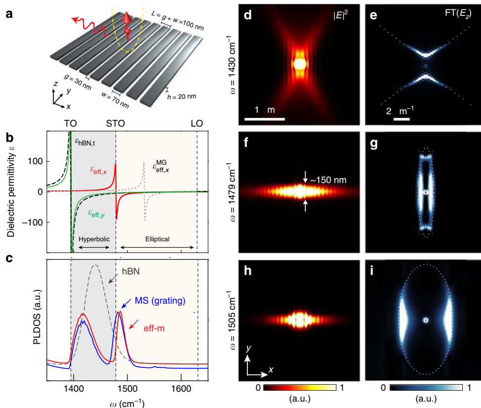
Fig. 1 Topological transition and canalization of polaritons in a hBN metasurface. a Schematic of a 20-nm-thick hBN metasurface based on a grating made of nanoribbons. b Anisotropic effective dielectric permittivities (real parts) of the metasurface calculated using Eqs. 1–3, \epsilon_{\text{eff},x} (red line) and \epsilon_{\text{eff},y} (green). Permittivity of unpatterned hBN ( \epsilon_{\text{hBN},t} , dashed black line) and effective permittivity of the metasurface based on Maxwell-Garnett approximation ( \epsilon_{\text{eff},x}^{\text{MG}} , dashed gray line) are provided for comparison. c Simulated PLDOS on the grating metasurface (MS), the effective medium (eff-m) and the unpatterned hBN, respectively. d, f, h Near-field intensity distribution of dipole-launched polaritons at three different frequencies. e, g, i Absolute value of the Fourier transform (FT) of the simulated near-field distribution E_z (see Supplementary Fig. 4). Dotted hyperbola and ellipses are guides to the eye.
