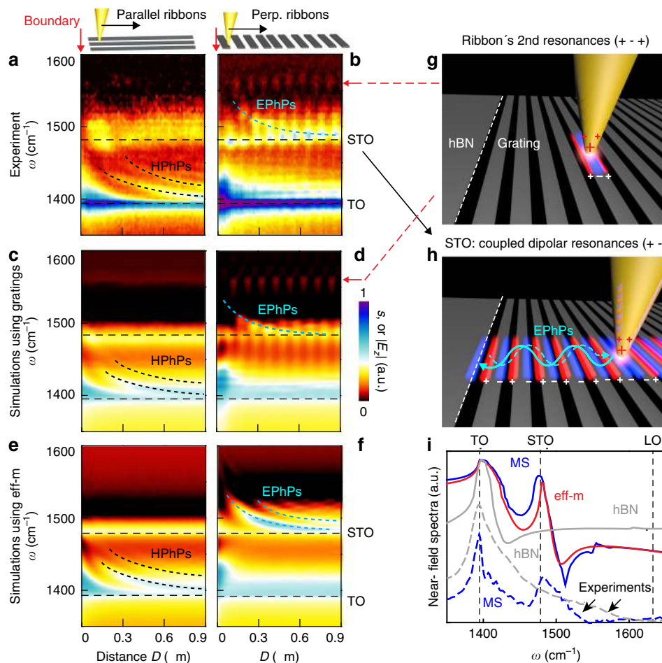
Fig. 3 Hyperspectral nanoimaging of polariton evolution in a hBN metasurface. Near-field spectroscopic line scans taken parallel (a) and perpendicular (b) to the ribbons, as indicated in the top schematics. c–f Simulated line scans based on two different models, c, d for real grating structures, e, f for the effective medium (eff-m). g, h Schematics of tip-excitation of the second- and first-order dipolar PhP resonances of the hBN ribbons, respectively. i Dashed lines show experimental near-field spectra taken from the metasurface (on a gap of the grating, dashed blue line) and on the unstructured hBN (dashed gray line). Solid lines show simulated near-field spectra of the grating (blue line), of eff-m (red line) and of the unstructured hBN (gray line).
