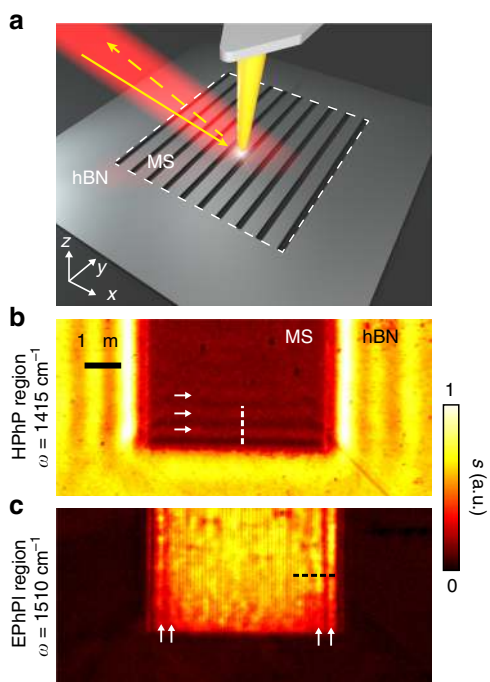
Fig. 2 Near-field imaging of polariton evolution in a hBN metasurface.
